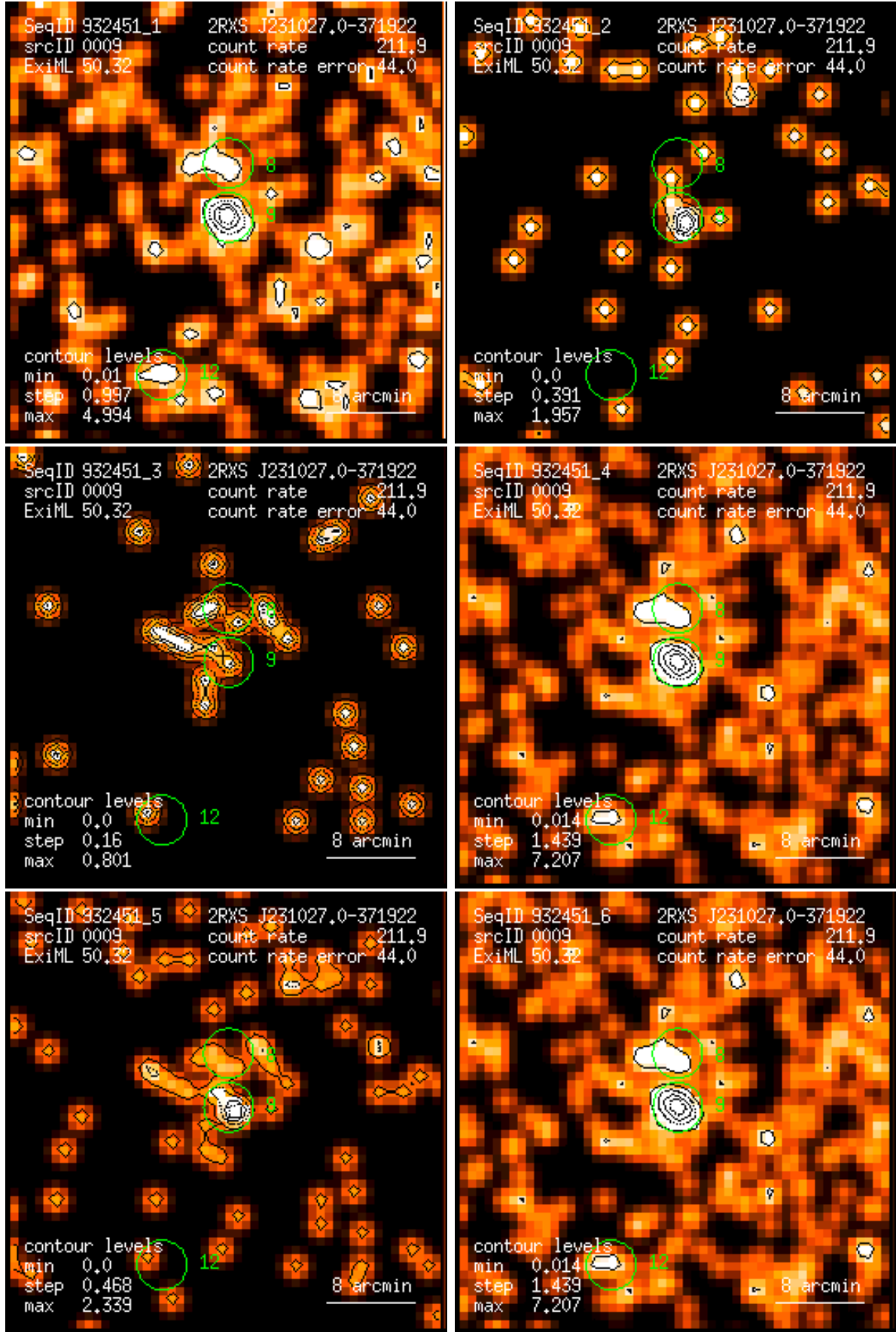
Figure 9: RASS 932451: detection 0009: band rate images, Gaussian filter: (1) PSPC channels 11 – 41, (2) 52 – 90, (3) 91 – 201, (4) 11 – 235, (5) 52 – 201, (6) 11 – 201. Broad band rates in counts/ks. Band rate contour levels in counts/ks/arcmin 2 .
