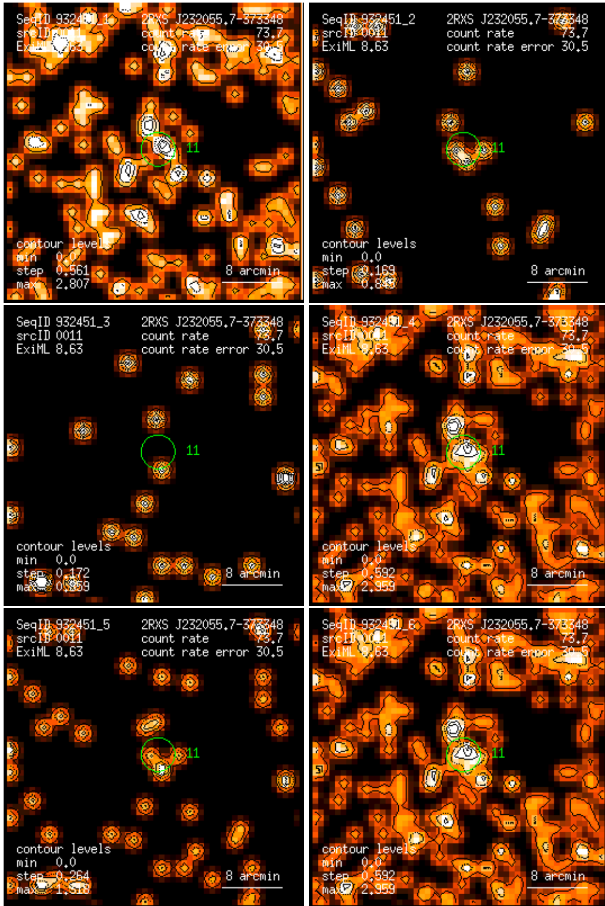
Figure 11: RASS 932451: detection 0011: band rate images, Gaussian filter: (1) PSPC channels 11 – 41, (2) 52 – 90, (3) 91 – 201, (4) 11 – 235, (5) 52 – 201, (6) 11 – 201. Broad band rates in counts/ks. Band rate contour levels in counts/ks/arcmin 2 .
