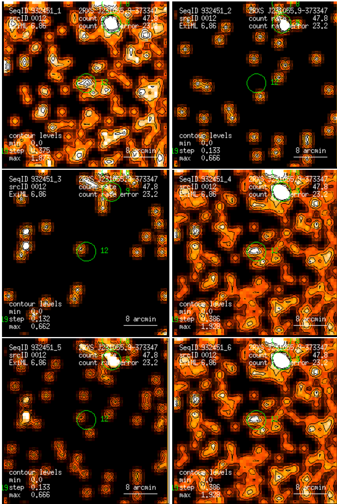
Figure 12: RASS 932451: detection 0012: band rate images, Gaussian filter: (1) PSPC channels 11 – 41, (2) 52 – 90, (3) 91 – 201, (4) 11 – 235, (5) 52 – 201, (6) 11 – 201. Broad band rates in counts/ks. Band rate contour levels in counts/ks/arcmin 2 .
