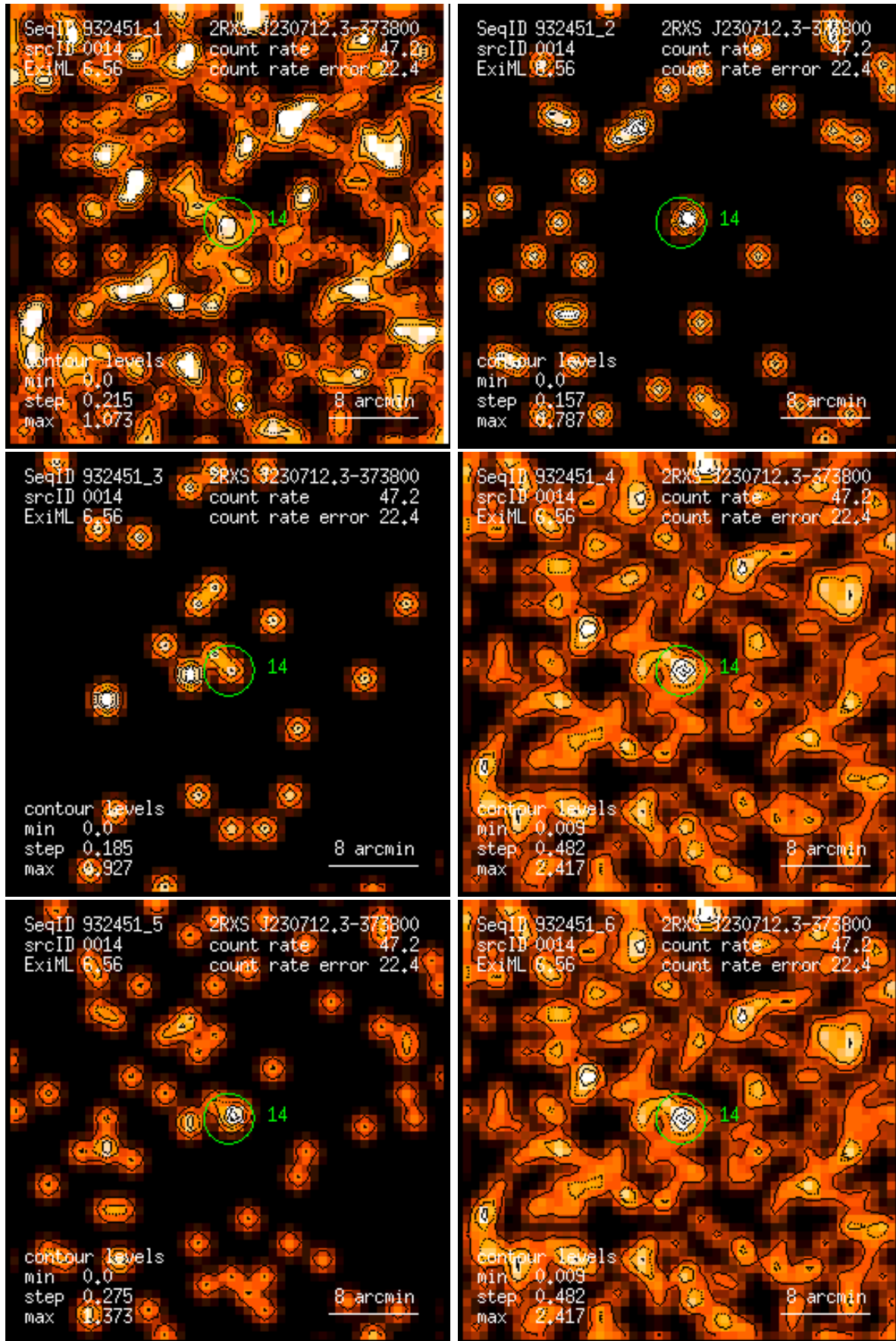
Figure 14: RASS 932451: detection 0014: band rate images, Gaussian filter: (1) PSPC channels 11 – 41, (2) 52 – 90, (3) 91 – 201, (4) 11 – 235, (5) 52 – 201, (6) 11 – 201. Broad band rates in counts/ks. Band rate contour levels in counts/ks/arcmin 2 .
