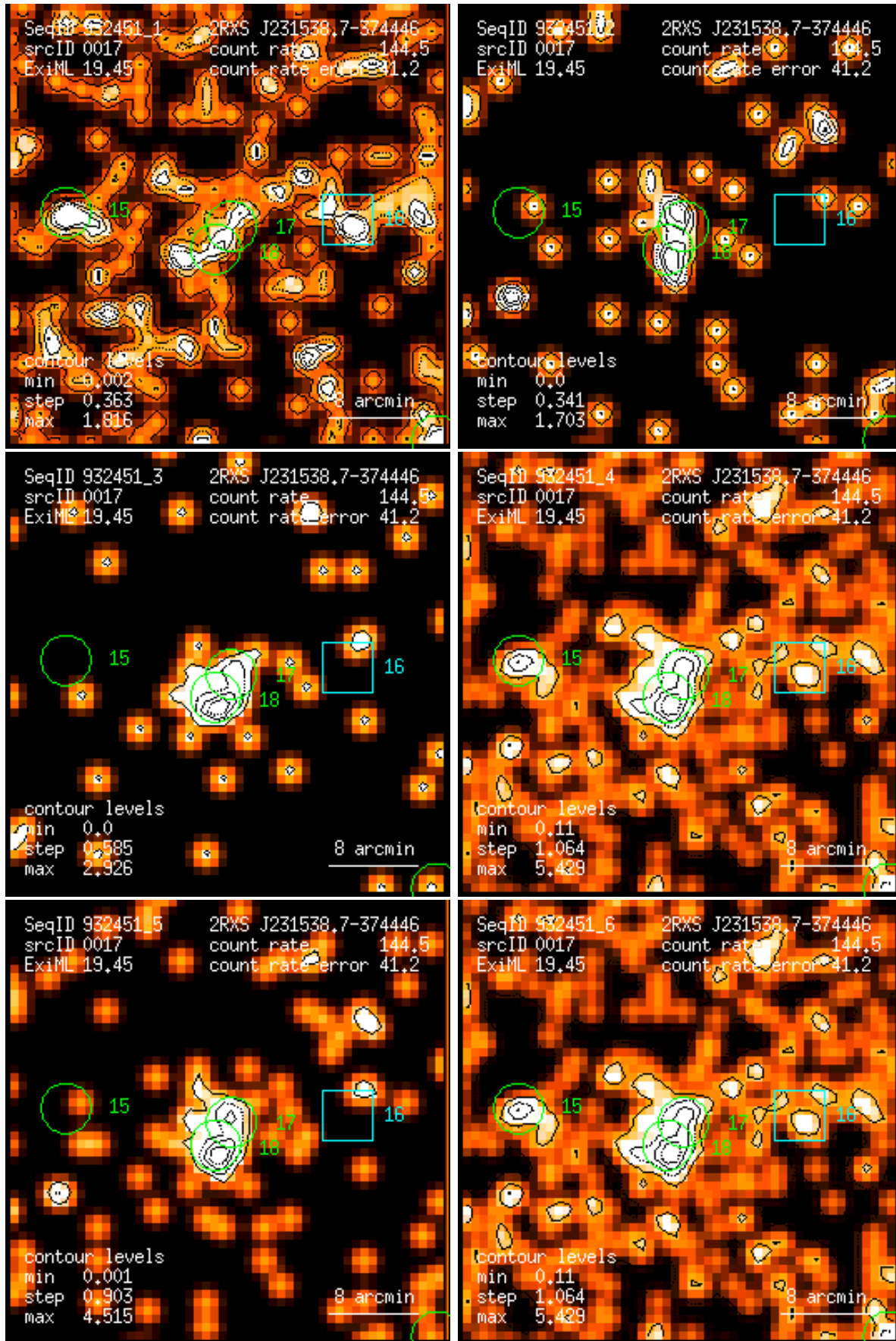
Figure 17: RASS 932451: detection 0017: band rate images, Gaussian filter: (1) PSPC channels 11 – 41, (2) 52 – 90, (3) 91 – 201, (4) 11 – 235, (5) 52 – 201, (6) 11 – 201. Broad band rates in counts/ks. Band rate contour levels in counts/ks/arcmin 2 .
