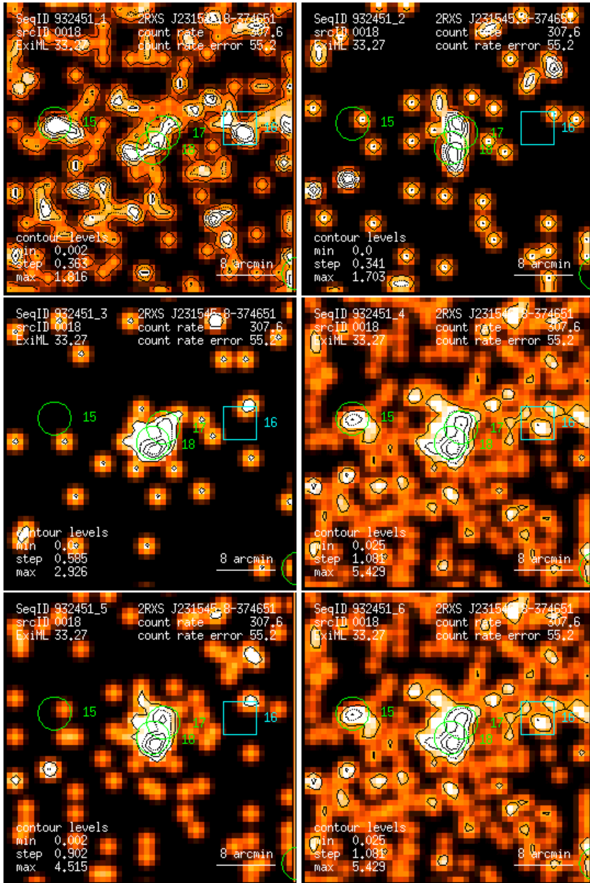
Figure 18: RASS 932451: detection 0018: band rate images, Gaussian filter: (1) PSPC channels 11 – 41, (2) 52 – 90, (3) 91 – 201, (4) 11 – 235, (5) 52 – 201, (6) 11 – 201. Broad band rates in counts/ks. Band rate contour levels in counts/ks/arcmin 2 .
