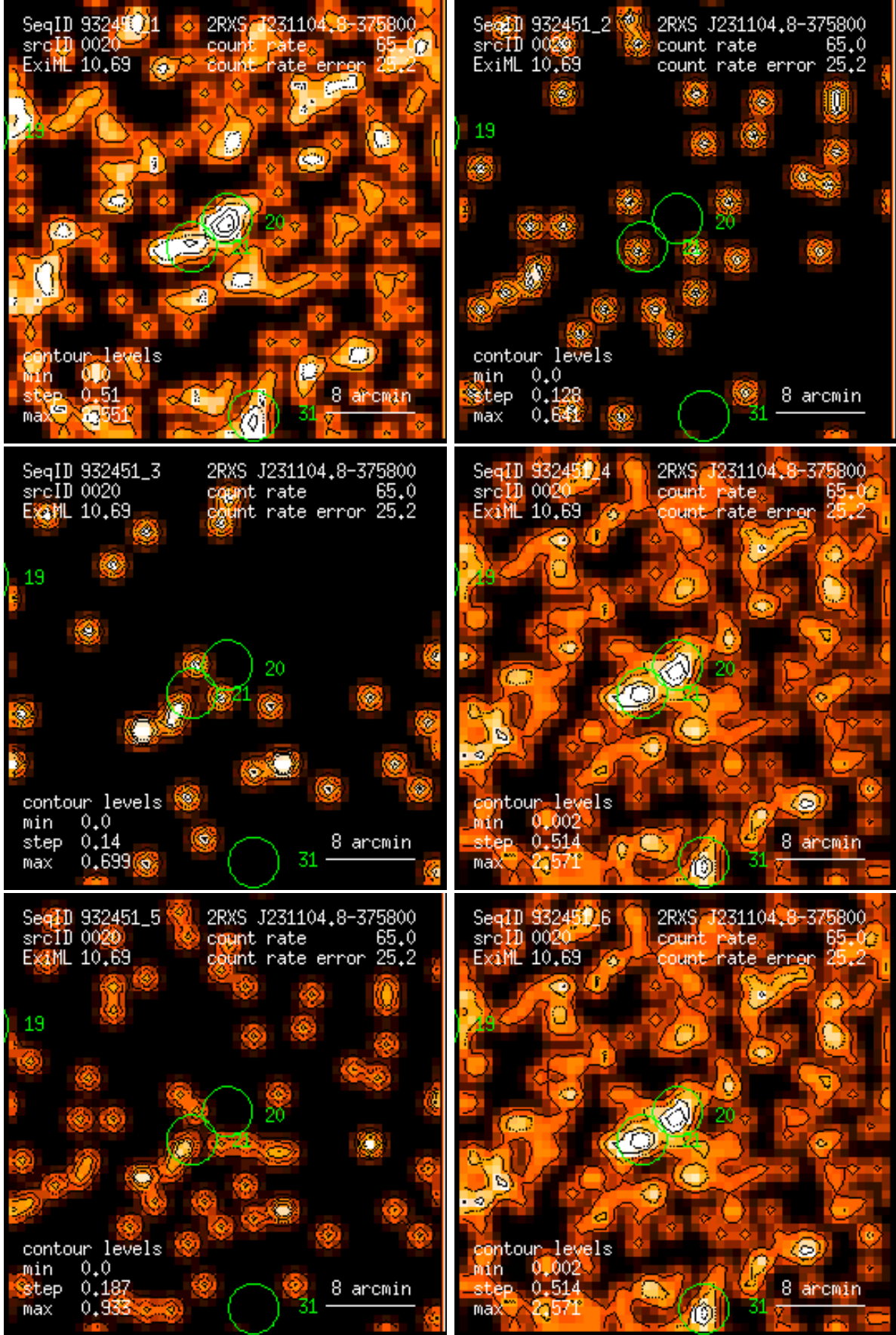
Figure 20: RASS 932451: detection 0020: band rate images, Gaussian filter: (1) PSPC channels 11 – 41, (2) 52 – 90, (3) 91 – 201, (4) 11 – 235, (5) 52 – 201, (6) 11 – 201. Broad band rates in counts/ks. Band rate contour levels in counts/ks/arcmin 2 .
