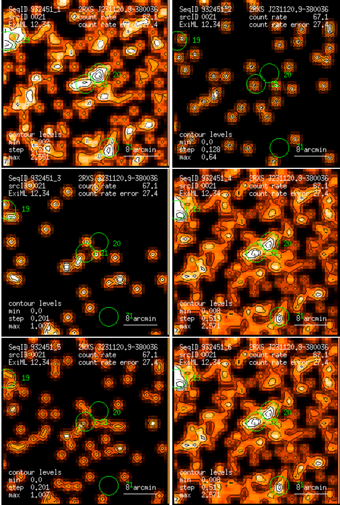
Figure 21: RASS 932451: detection 0021: band rate images, Gaussian filter: (1) PSPC channels 11 – 41, (2) 52 – 90, (3) 91 – 201, (4) 11 – 235, (5) 52 – 201, (6) 11 – 201. Broad band rates in counts/ks. Band rate contour levels in counts/ks/arcmin 2 .
