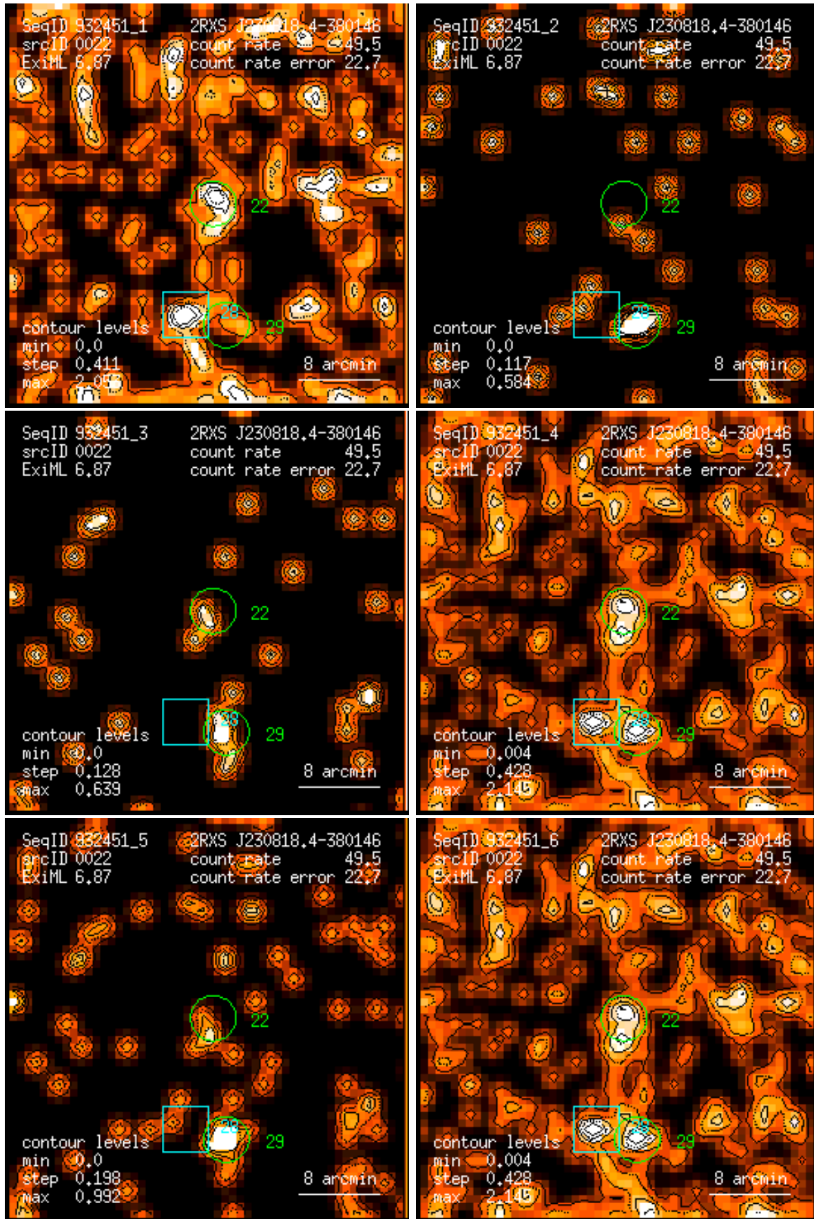
Figure 22: RASS 932451: detection 0022: band rate images, Gaussian filter: (1) PSPC channels 11 – 41, (2) 52 – 90, (3) 91 – 201, (4) 11 – 235, (5) 52 – 201, (6) 11 – 201. Broad band rates in counts/ks. Band rate contour levels in counts/ks/arcmin 2 .
