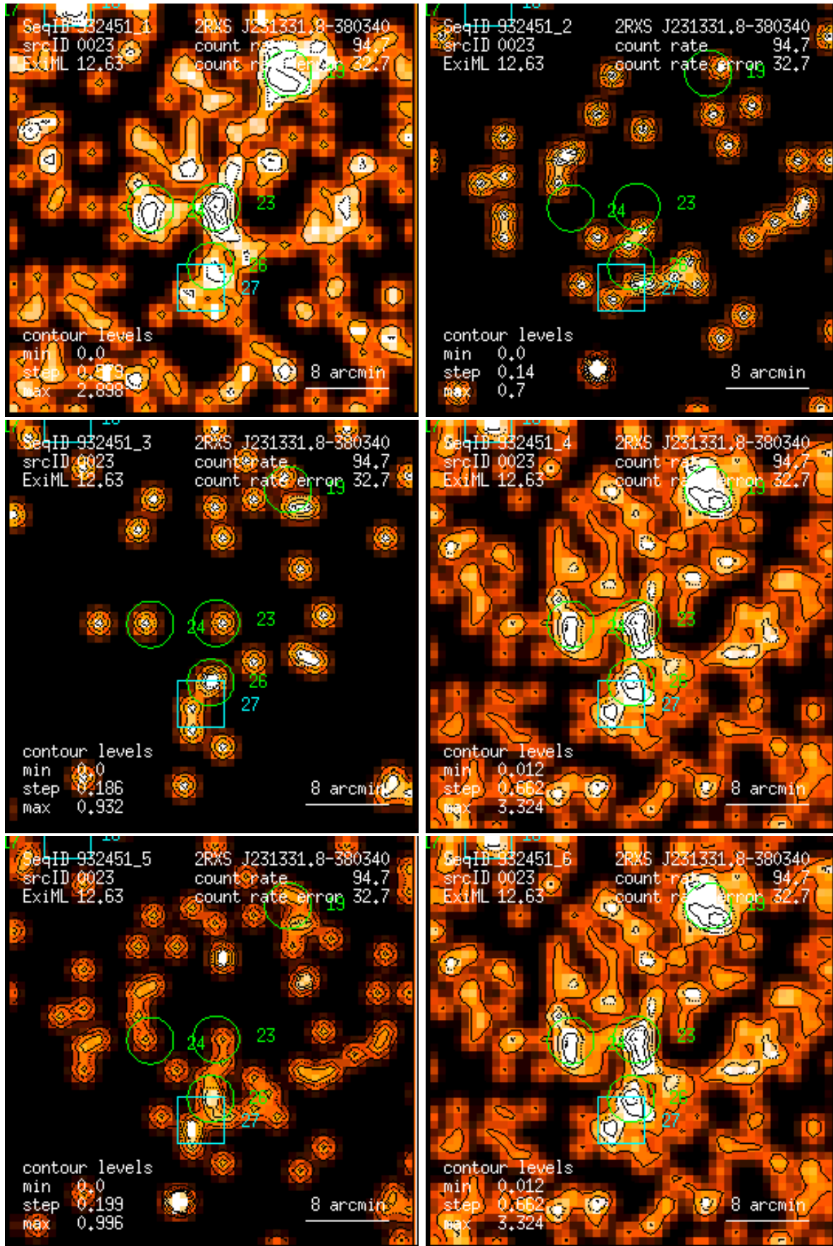
Figure 23: RASS 932451: detection 0023: band rate images, Gaussian filter: (1) PSPC channels 11 – 41, (2) 52 – 90, (3) 91 – 201, (4) 11 – 235, (5) 52 – 201, (6) 11 – 201. Broad band rates in counts/ks. Band rate contour levels in counts/ks/arcmin 2 .
