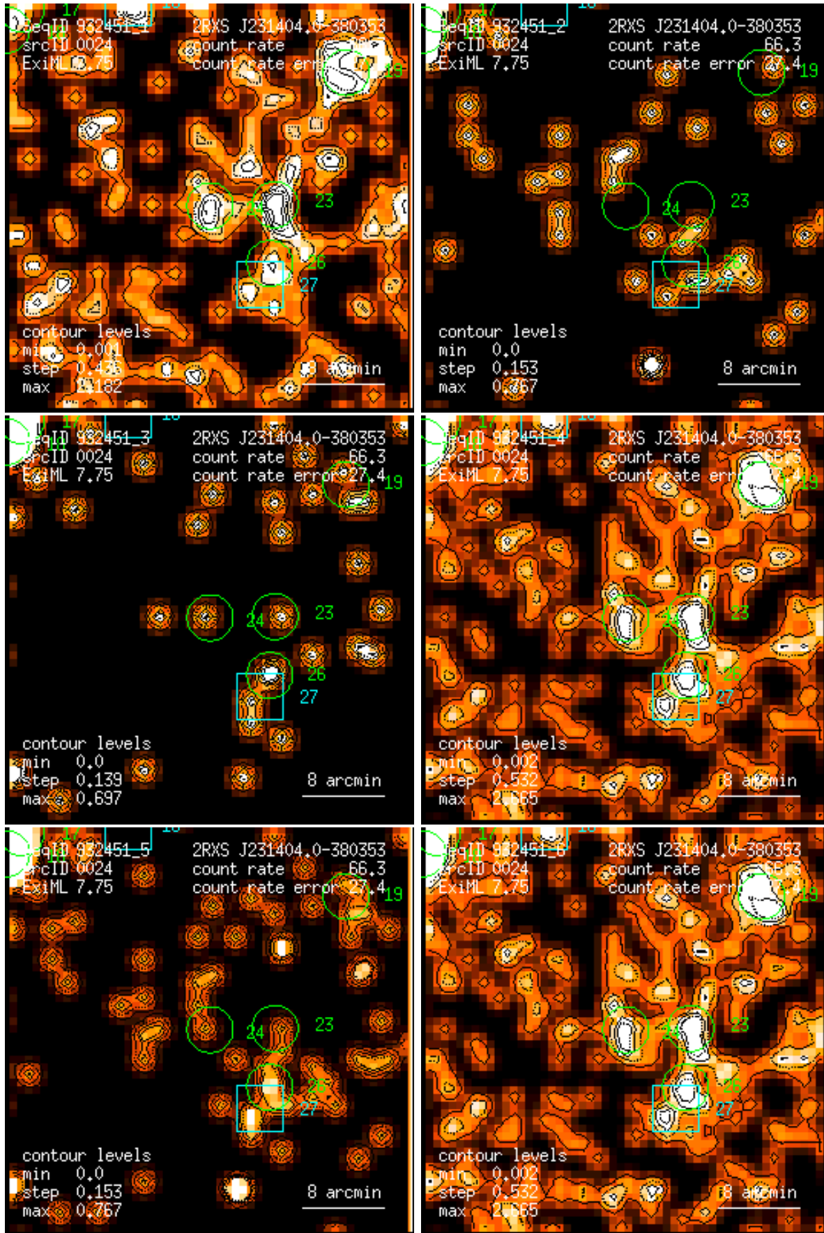
Figure 24: RASS 932451: detection 0024: band rate images, Gaussian filter: (1) PSPC channels 11 – 41, (2) 52 – 90, (3) 91 – 201, (4) 11 – 235, (5) 52 – 201, (6) 11 – 201. Broad band rates in counts/ks. Band rate contour levels in counts/ks/arcmin 2 .
