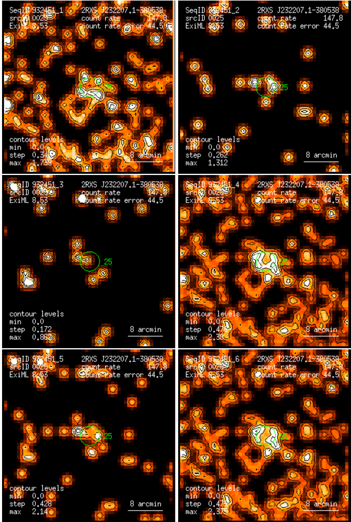
Figure 25: RASS 932451: detection 0025: band rate images, Gaussian filter: (1) PSPC channels 11 – 41, (2) 52 – 90, (3) 91 – 201, (4) 11 – 235, (5) 52 – 201, (6) 11 – 201. Broad band rates in counts/ks. Band rate contour levels in counts/ks/arcmin 2 .
