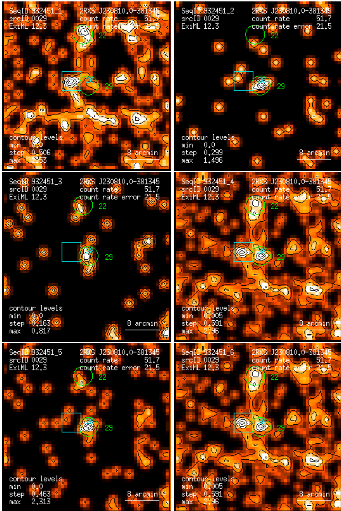
Figure 29: RASS 932451: detection 0029: band rate images, Gaussian filter: (1) PSPC channels 11 – 41, (2) 52 – 90, (3) 91 – 201, (4) 11 – 235, (5) 52 – 201, (6) 11 – 201. Broad band rates in counts/ks. Band rate contour levels in counts/ks/arcmin 2 .
