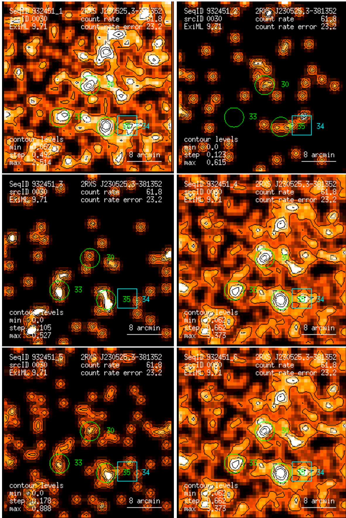
Figure 30: RASS 932451: detection 0030: band rate images, Gaussian filter: (1) PSPC channels 11 – 41, (2) 52 – 90, (3) 91 – 201, (4) 11 – 235, (5) 52 – 201, (6) 11 – 201. Broad band rates in counts/ks. Band rate contour levels in counts/ks/arcmin 2 .
