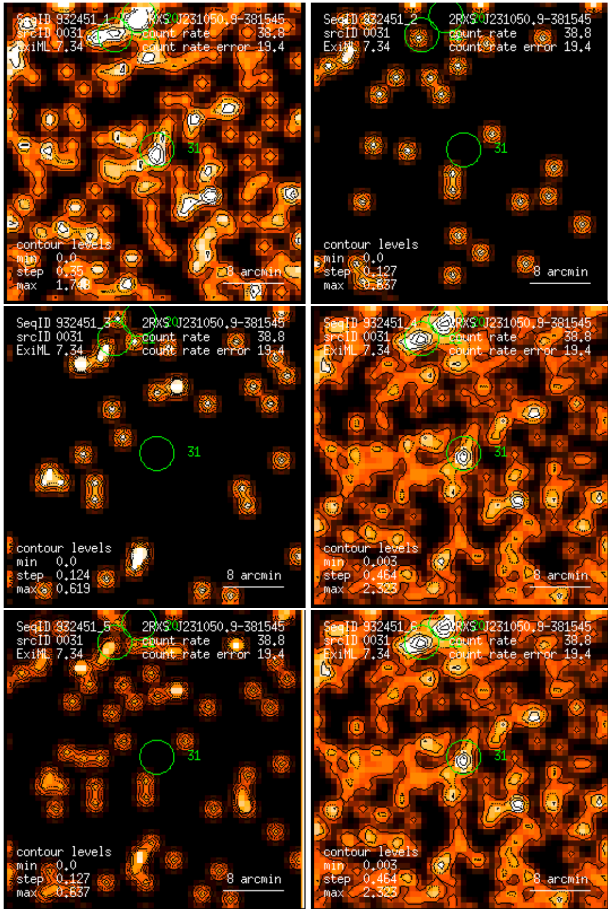
Figure 31: RASS 932451: detection 0031: band rate images, Gaussian filter: (1) PSPC channels 11 – 41, (2) 52 – 90, (3) 91 – 201, (4) 11 – 235, (5) 52 – 201, (6) 11 – 201. Broad band rates in counts/ks. Band rate contour levels in counts/ks/arcmin 2 .
