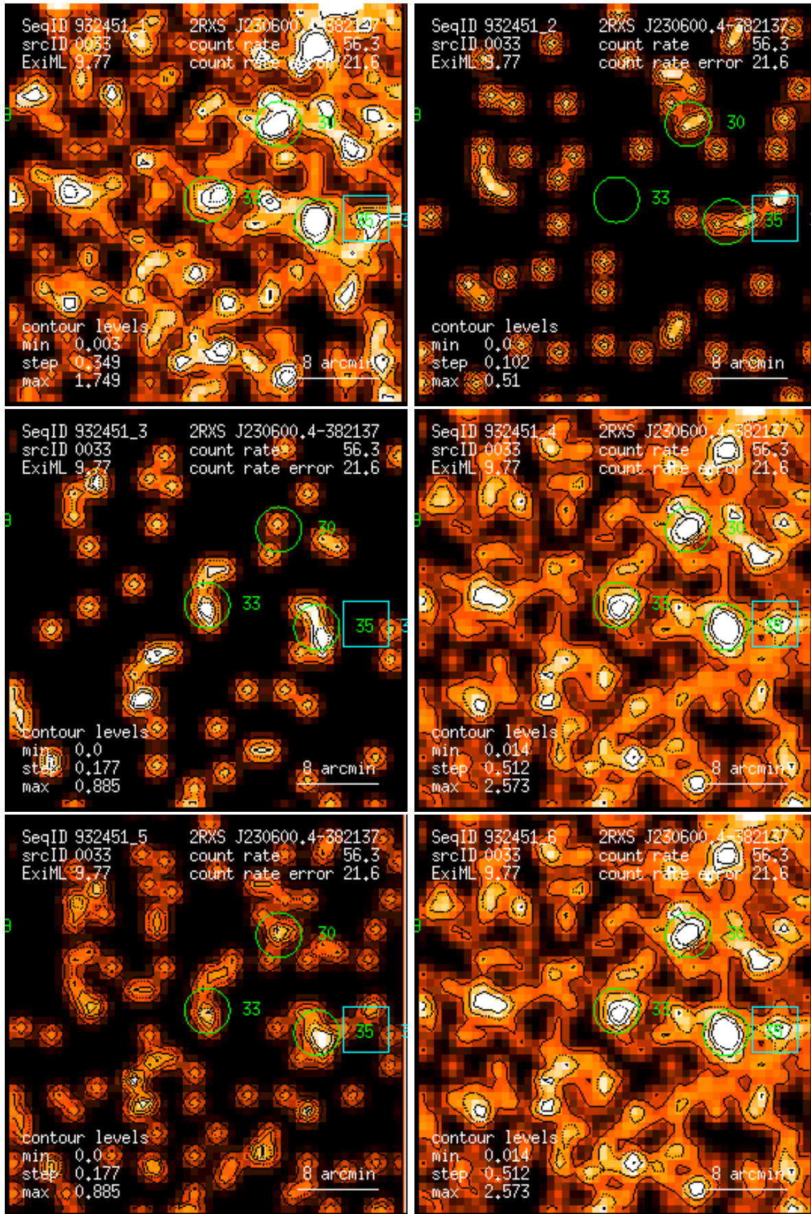
Figure 33: RASS 932451: detection 0033: band rate images, Gaussian filter: (1) PSPC channels 11 – 41, (2) 52 – 90, (3) 91 – 201, (4) 11 – 235, (5) 52 – 201, (6) 11 – 201. Broad band rates in counts/ks. Band rate contour levels in counts/ks/arcmin 2 .
