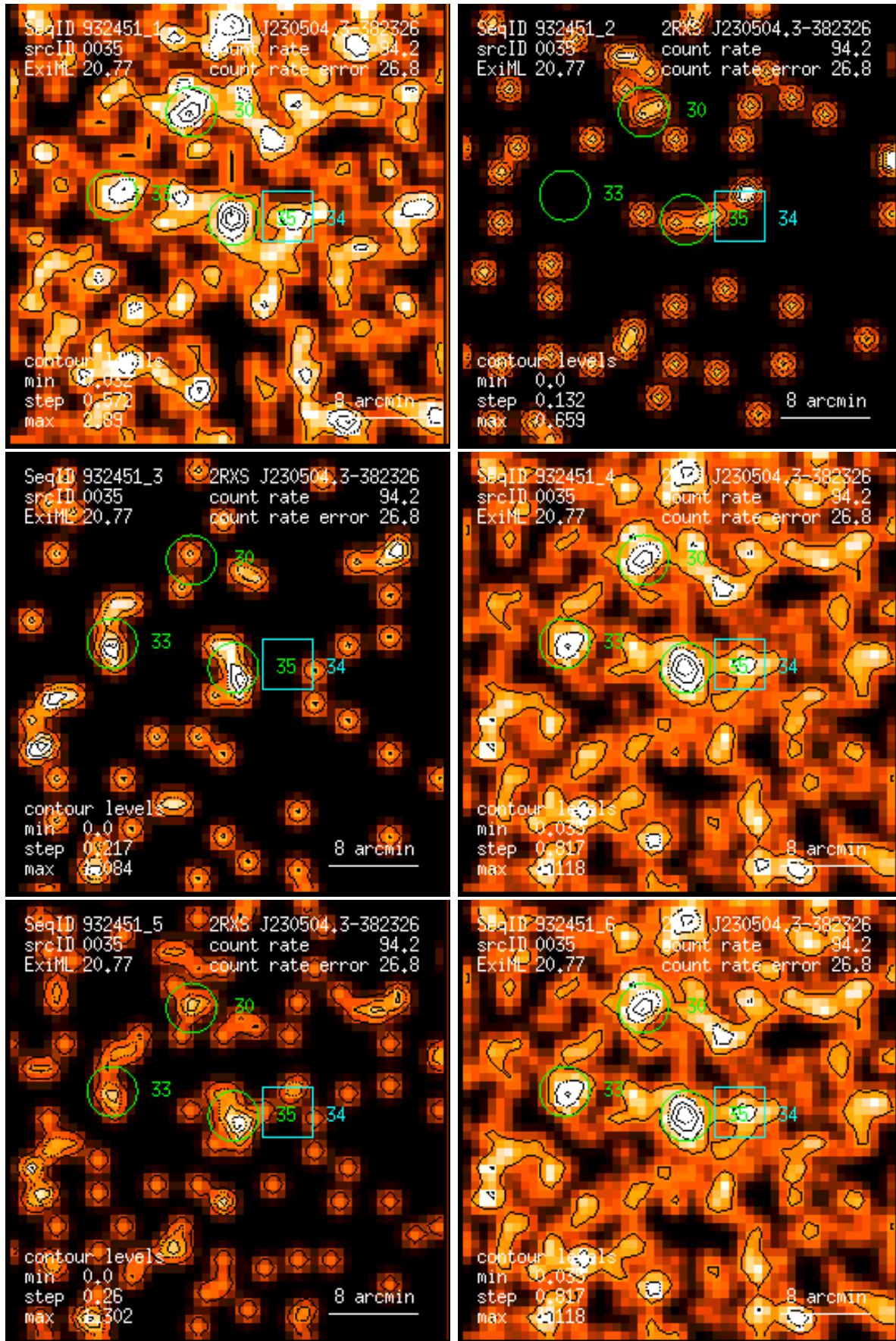
Figure 35: RASS 932451: detection 0035: band rate images, Gaussian filter: (1) PSPC channels 11 – 41, (2) 52 – 90, (3) 91 – 201, (4) 11 – 235, (5) 52 – 201, (6) 11 – 201. Broad band rates in counts/ks. Band rate contour levels in counts/ks/arcmin 2 .
