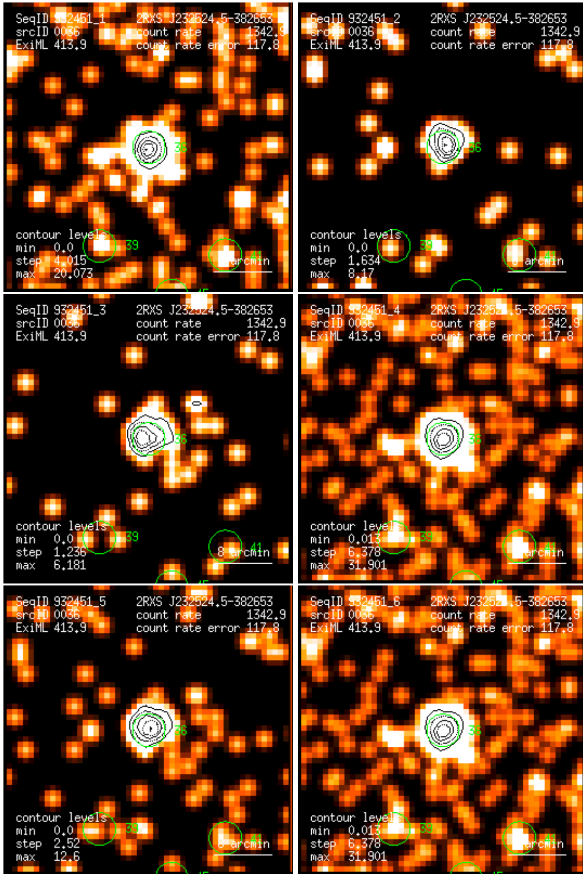
Figure 36: RASS 932451: detection 0036: band rate images, Gaussian filter: (1) PSPC channels 11 – 41, (2) 52 – 90, (3) 91 – 201, (4) 11 – 235, (5) 52 – 201, (6) 11 – 201. Broad band rates in counts/ks. Band rate contour levels in counts/ks/arcmin 2 .
