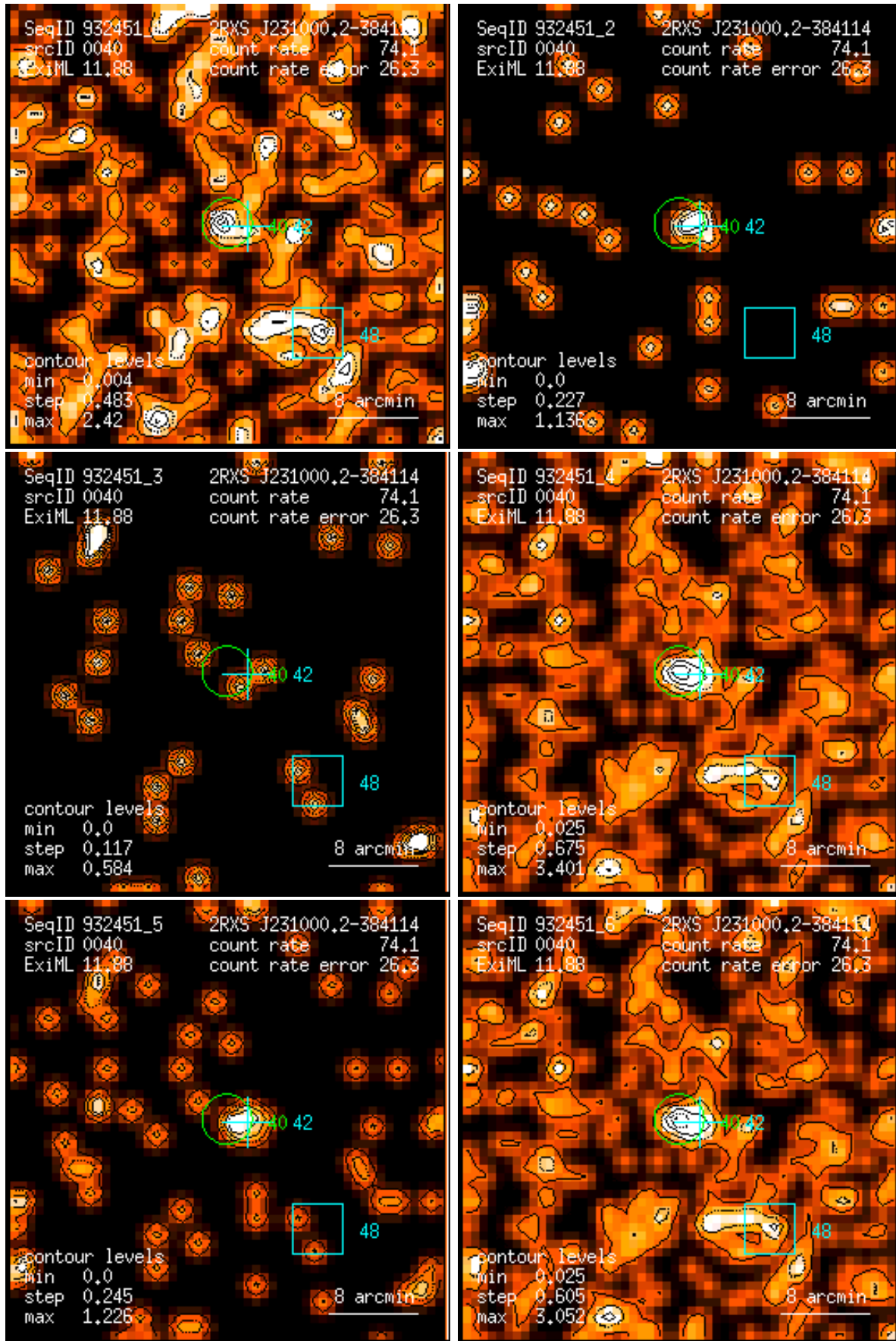
Figure 40: RASS 932451: detection 0040: band rate images, Gaussian filter: (1) PSPC channels 11 – 41, (2) 52 – 90, (3) 91 – 201, (4) 11 – 235, (5) 52 – 201, (6) 11 – 201. Broad band rates in counts/ks. Band rate contour levels in counts/ks/arcmin 2 .
