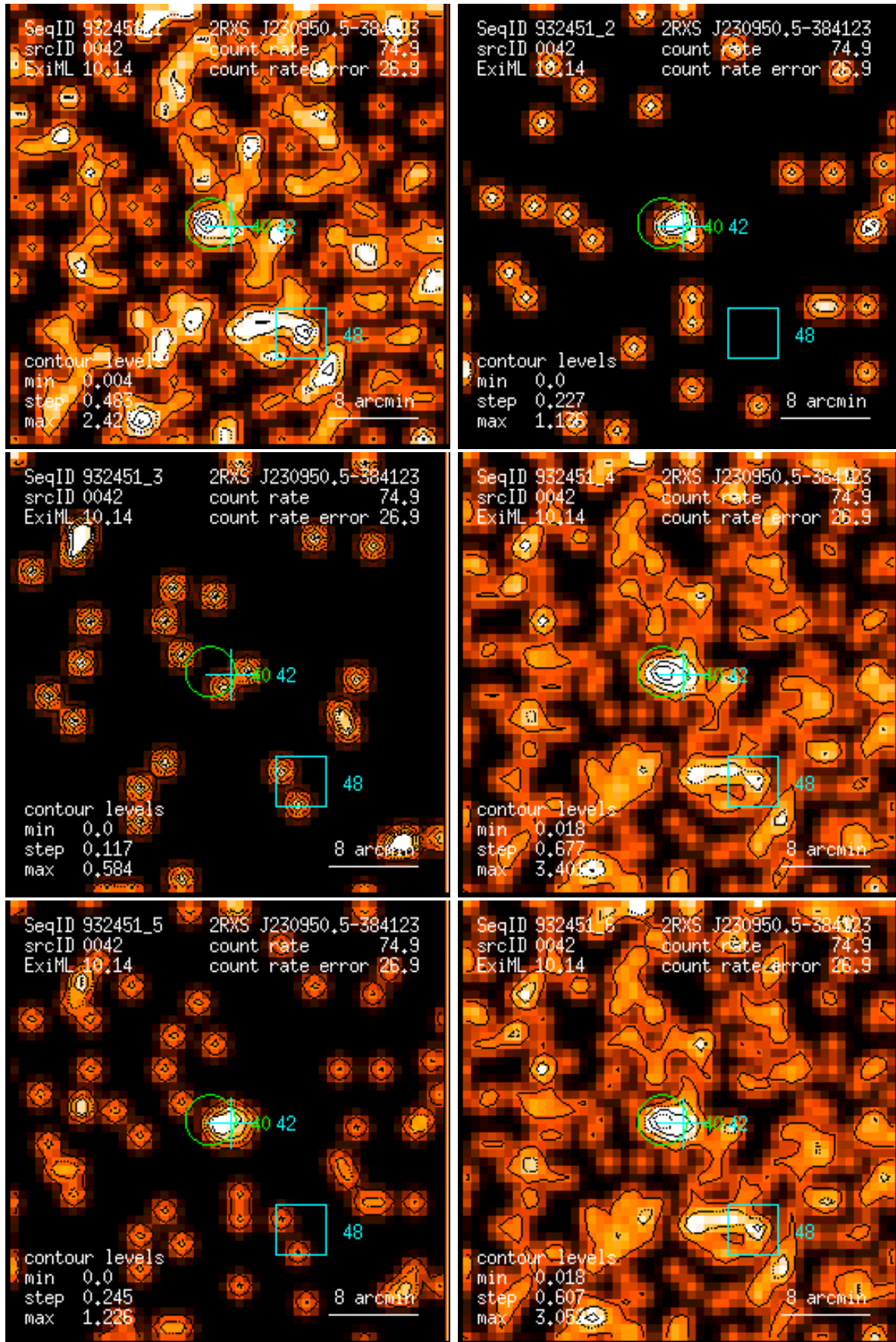
Figure 42: RASS 932451: detection 0042: band rate images, Gaussian filter: (1) PSPC channels 11 – 41, (2) 52 – 90, (3) 91 – 201, (4) 11 – 235, (5) 52 – 201, (6) 11 – 201. Broad band rates in counts/ks. Band rate contour levels in counts/ks/arcmin 2 .
