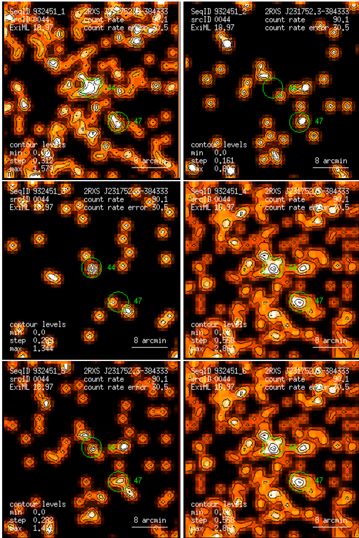
Figure 44: RASS 932451: detection 0044: band rate images, Gaussian filter: (1) PSPC channels 11 – 41, (2) 52 – 90, (3) 91 – 201, (4) 11 – 235, (5) 52 – 201, (6) 11 – 201. Broad band rates in counts/ks. Band rate contour levels in counts/ks/arcmin 2 .
