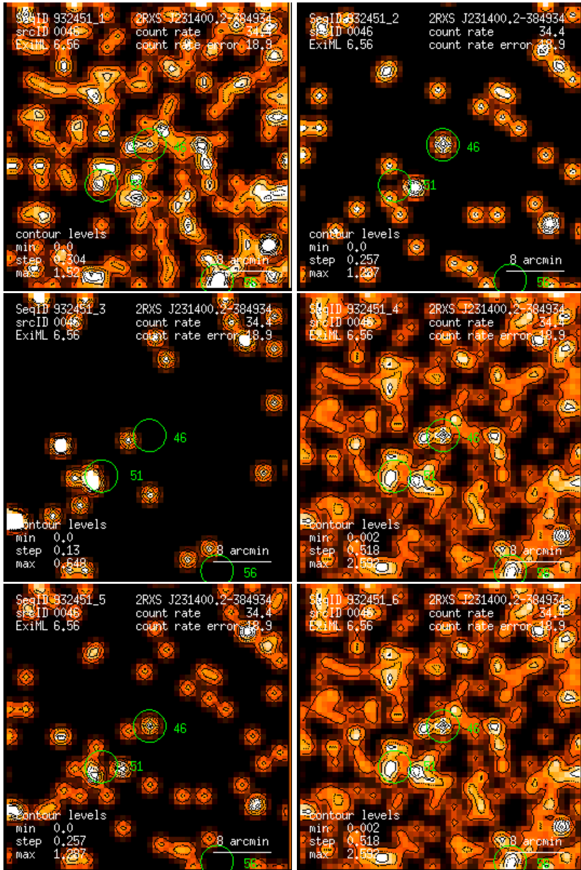
Figure 46: RASS 932451: detection 0046: band rate images, Gaussian filter: (1) PSPC channels 11 – 41, (2) 52 – 90, (3) 91 – 201, (4) 11 – 235, (5) 52 – 201, (6) 11 – 201. Broad band rates in counts/ks. Band rate contour levels in counts/ks/arcmin 2 .
