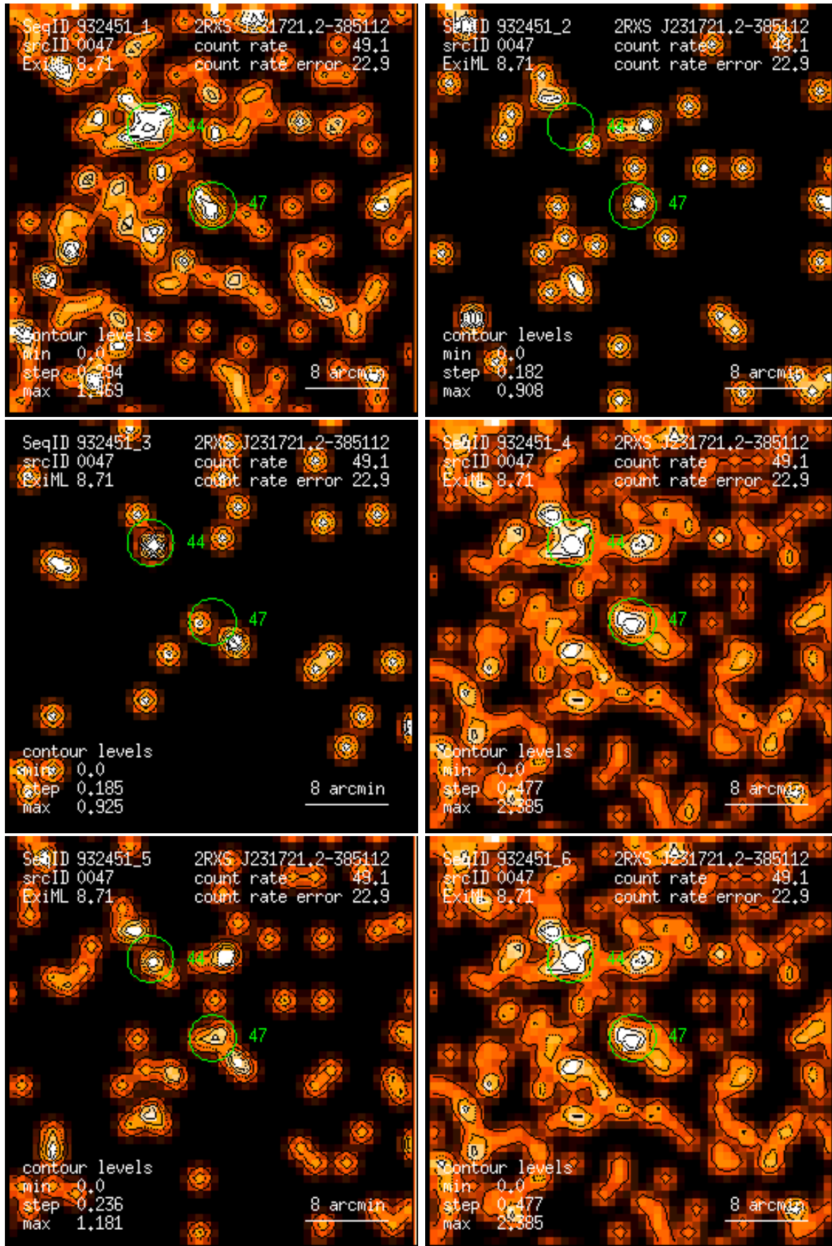
Figure 47: RASS 932451: detection 0047: band rate images, Gaussian filter: (1) PSPC channels 11 – 41, (2) 52 – 90, (3) 91 – 201, (4) 11 – 235, (5) 52 – 201, (6) 11 – 201. Broad band rates in counts/ks. Band rate contour levels in counts/ks/arcmin 2 .
