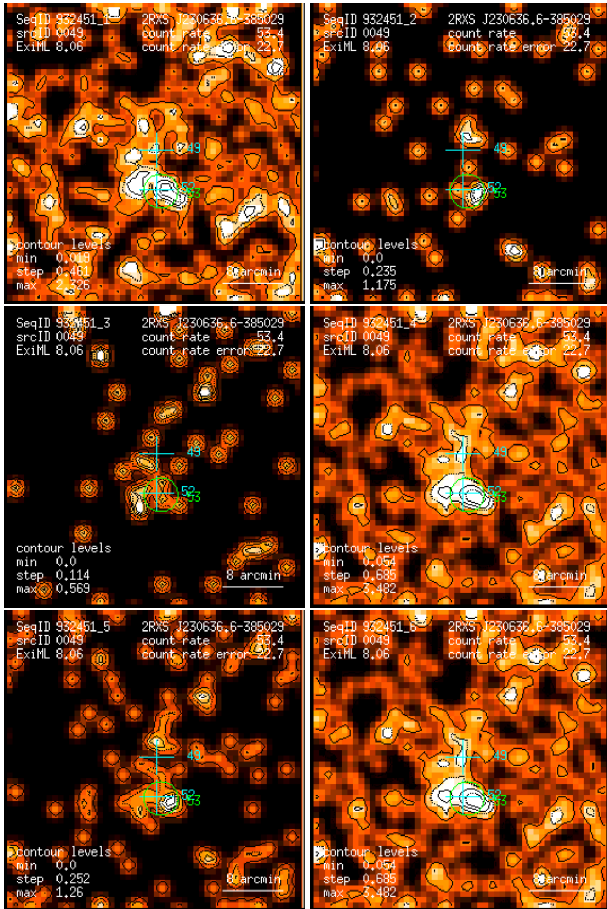
Figure 49: RASS 932451: detection 0049: band rate images, Gaussian filter: (1) PSPC channels 11 – 41, (2) 52 – 90, (3) 91 – 201, (4) 11 – 235, (5) 52 – 201, (6) 11 – 201. Broad band rates in counts/ks. Band rate contour levels in counts/ks/arcmin 2 .
