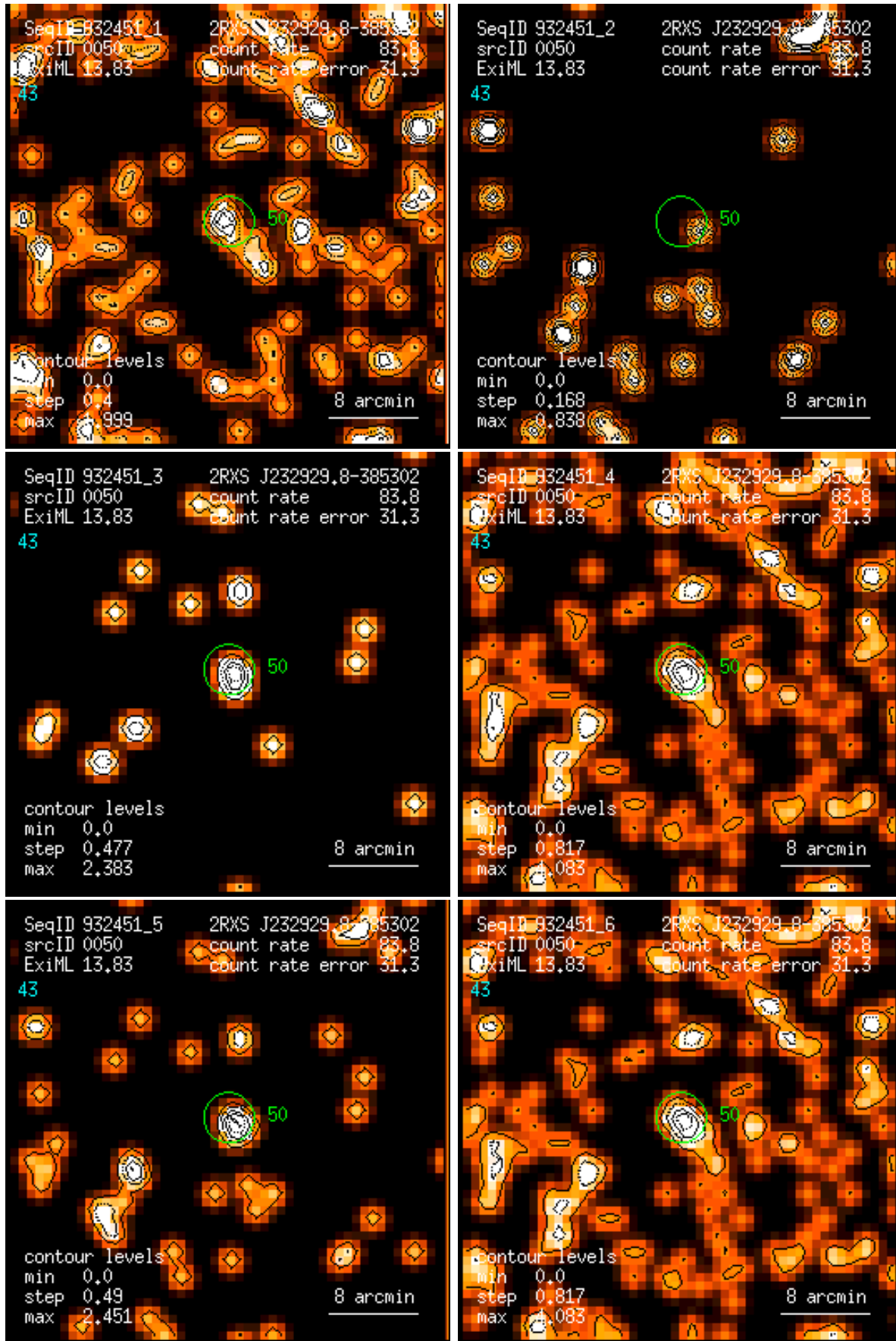
Figure 50: RASS 932451: detection 0050: band rate images, Gaussian filter: (1) PSPC channels 11 – 41, (2) 52 – 90, (3) 91 – 201, (4) 11 – 235, (5) 52 – 201, (6) 11 – 201. Broad band rates in counts/ks. Band rate contour levels in counts/ks/arcmin 2 .
