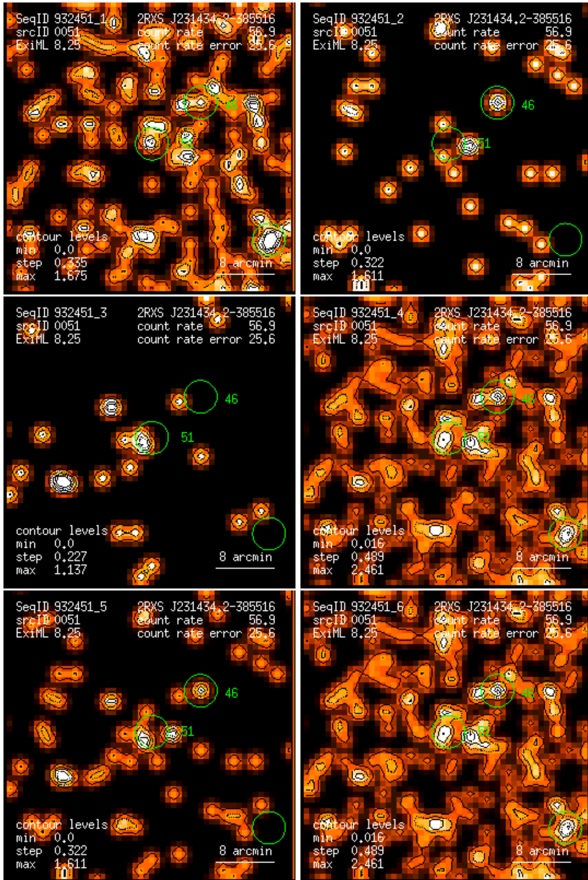
Figure 51: RASS 932451: detection 0051: band rate images, Gaussian filter: (1) PSPC channels 11 – 41, (2) 52 – 90, (3) 91 – 201, (4) 11 – 235, (5) 52 – 201, (6) 11 – 201. Broad band rates in counts/ks. Band rate contour levels in counts/ks/arcmin 2 .
