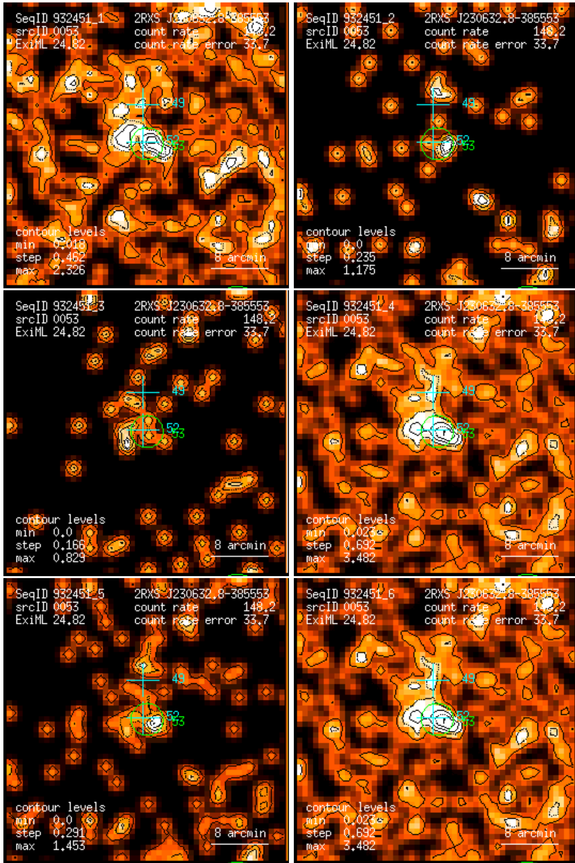
Figure 53: RASS 932451: detection 0053: band rate images, Gaussian filter: (1) PSPC channels 11 – 41, (2) 52 – 90, (3) 91 – 201, (4) 11 – 235, (5) 52 – 201, (6) 11 – 201. Broad band rates in counts/ks. Band rate contour levels in counts/ks/arcmin 2 .
