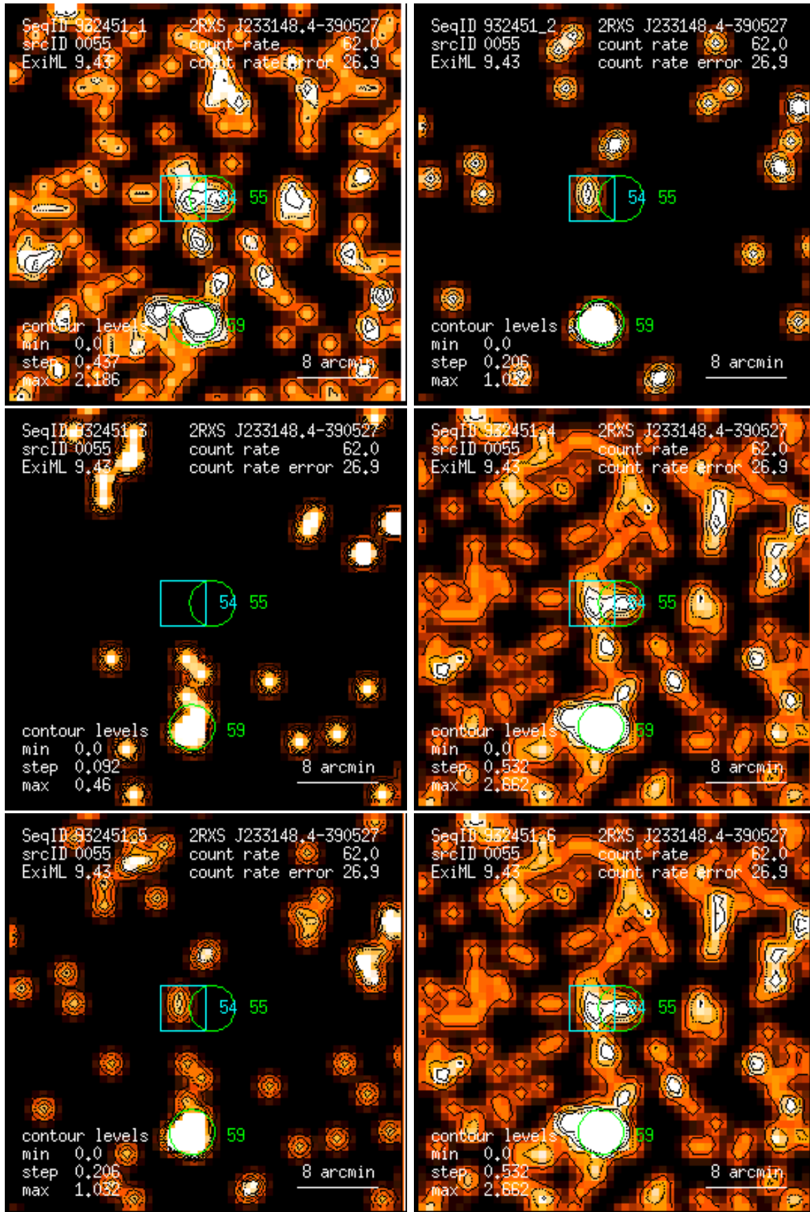
Figure 55: RASS 932451: detection 0055: band rate images, Gaussian filter: (1) PSPC channels 11 – 41, (2) 52 – 90, (3) 91 – 201, (4) 11 – 235, (5) 52 – 201, (6) 11 – 201. Broad band rates in counts/ks. Band rate contour levels in counts/ks/arcmin 2 .
