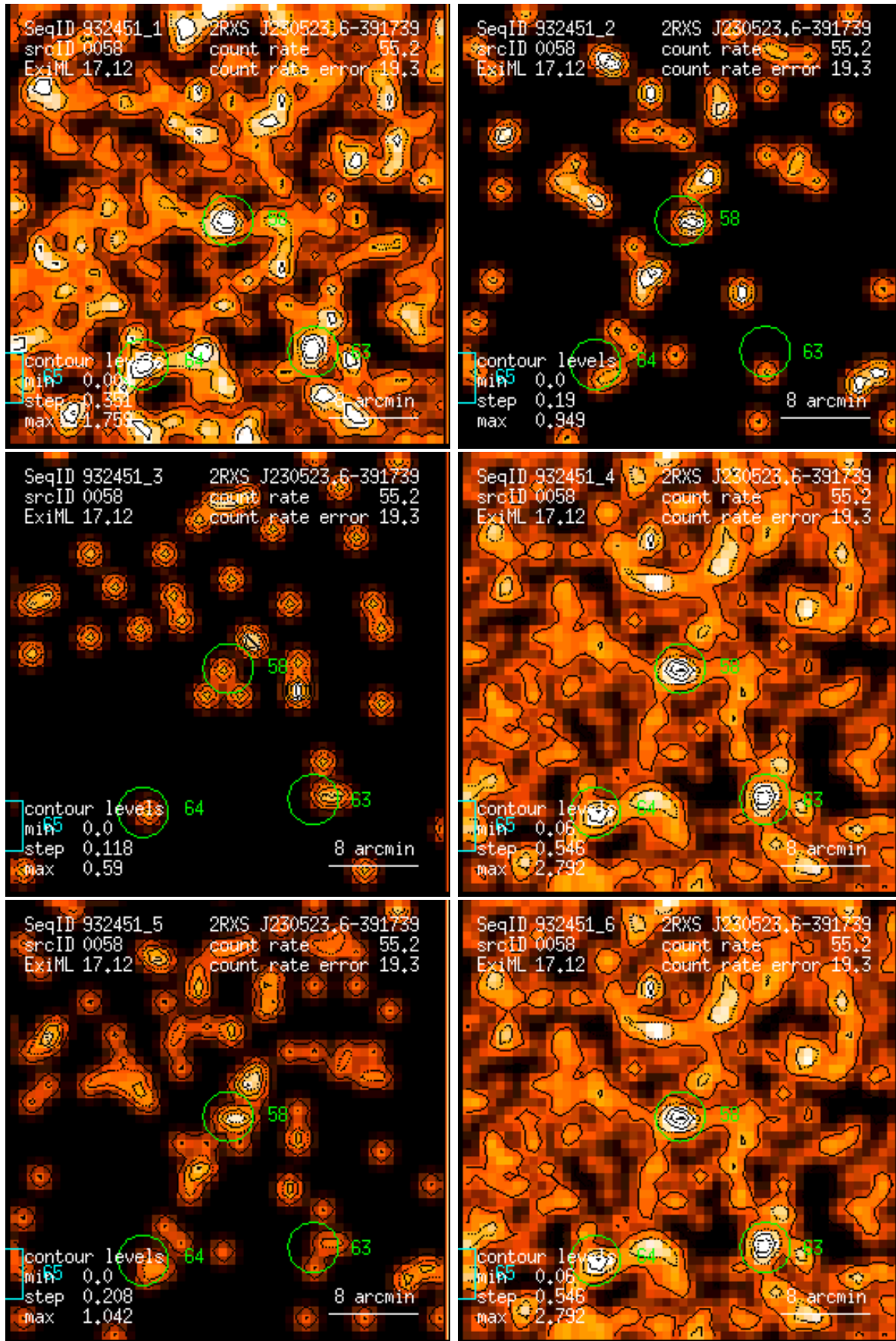
Figure 58: RASS 932451: detection 0058: band rate images, Gaussian filter: (1) PSPC channels 11 – 41, (2) 52 – 90, (3) 91 – 201, (4) 11 – 235, (5) 52 – 201, (6) 11 – 201. Broad band rates in counts/ks. Band rate contour levels in counts/ks/arcmin 2 .
