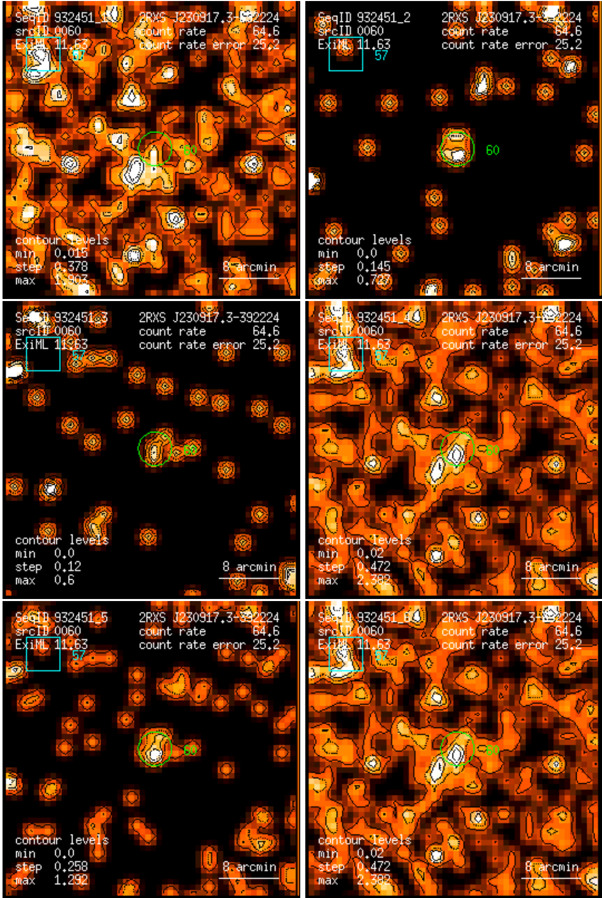
Figure 60: RASS 932451: detection 0060: band rate images, Gaussian filter: (1) PSPC channels 11 – 41, (2) 52 – 90, (3) 91 – 201, (4) 11 – 235, (5) 52 – 201, (6) 11 – 201. Broad band rates in counts/ks. Band rate contour levels in counts/ks/arcmin 2 .
