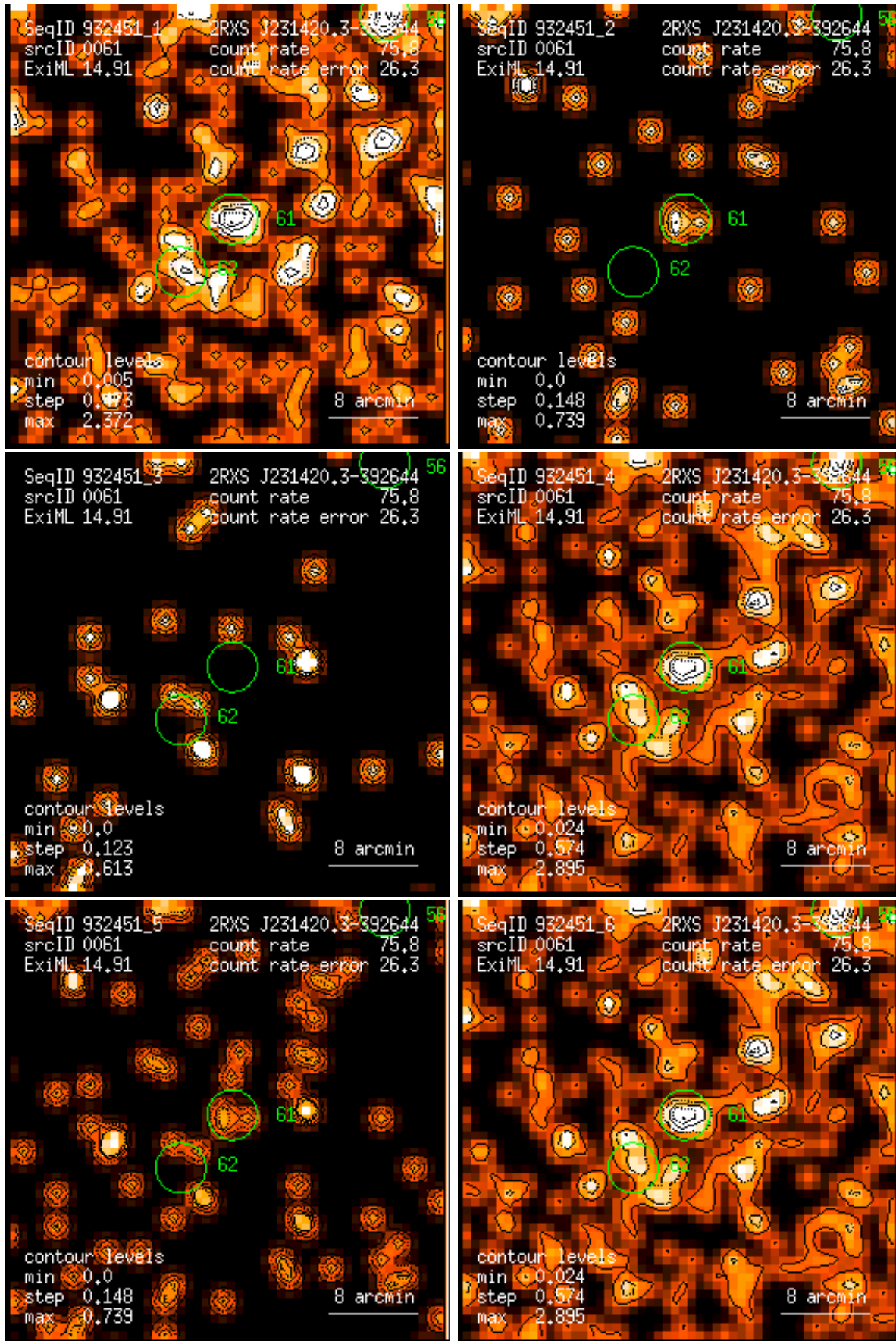
Figure 61: RASS 932451: detection 0061: band rate images, Gaussian filter: (1) PSPC channels 11 – 41, (2) 52 – 90, (3) 91 – 201, (4) 11 – 235, (5) 52 – 201, (6) 11 – 201. Broad band rates in counts/ks. Band rate contour levels in counts/ks/arcmin 2 .
