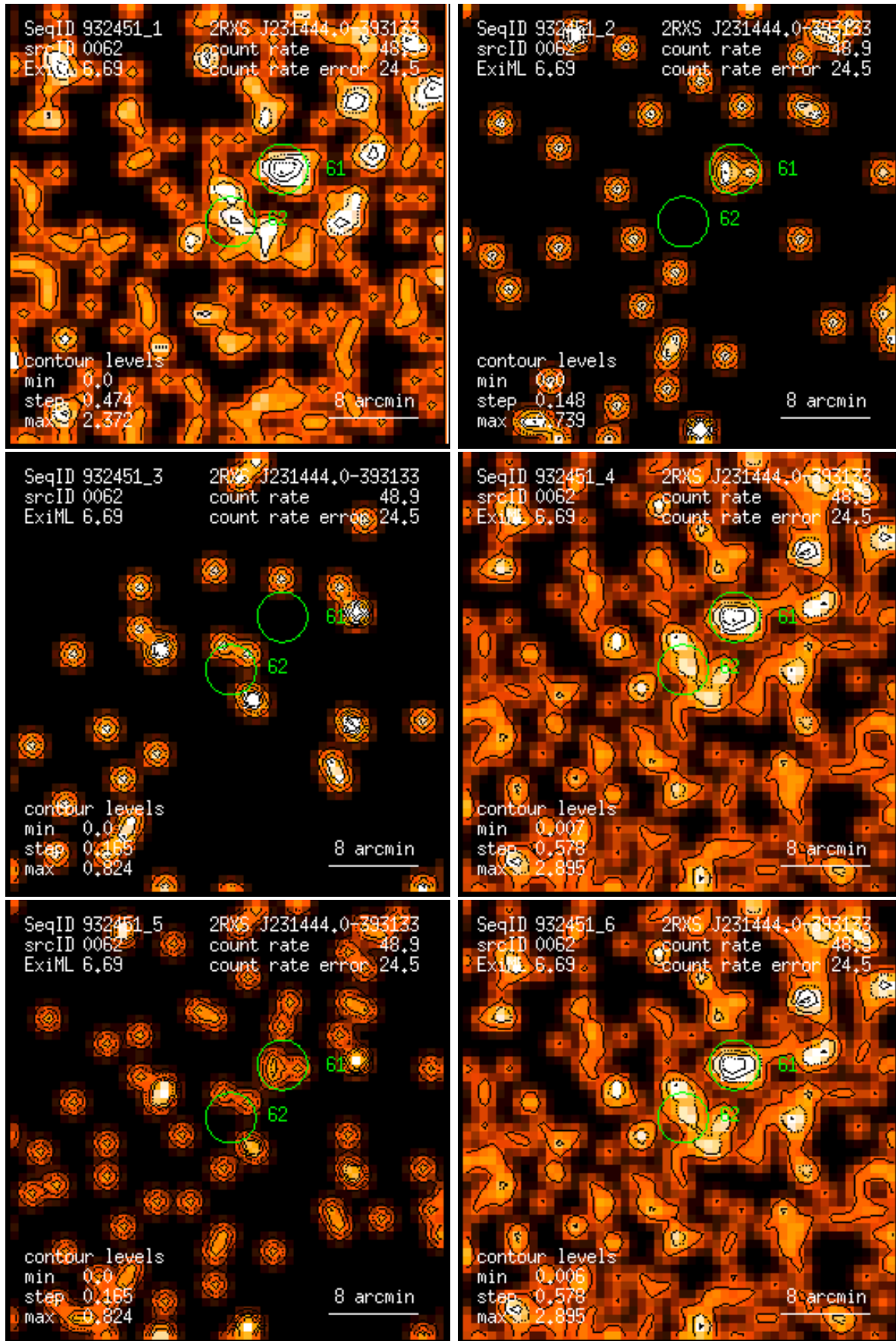
Figure 62: RASS 932451: detection 0062: band rate images, Gaussian filter: (1) PSPC channels 11 – 41, (2) 52 – 90, (3) 91 – 201, (4) 11 – 235, (5) 52 – 201, (6) 11 – 201. Broad band rates in counts/ks. Band rate contour levels in counts/ks/arcmin 2 .
