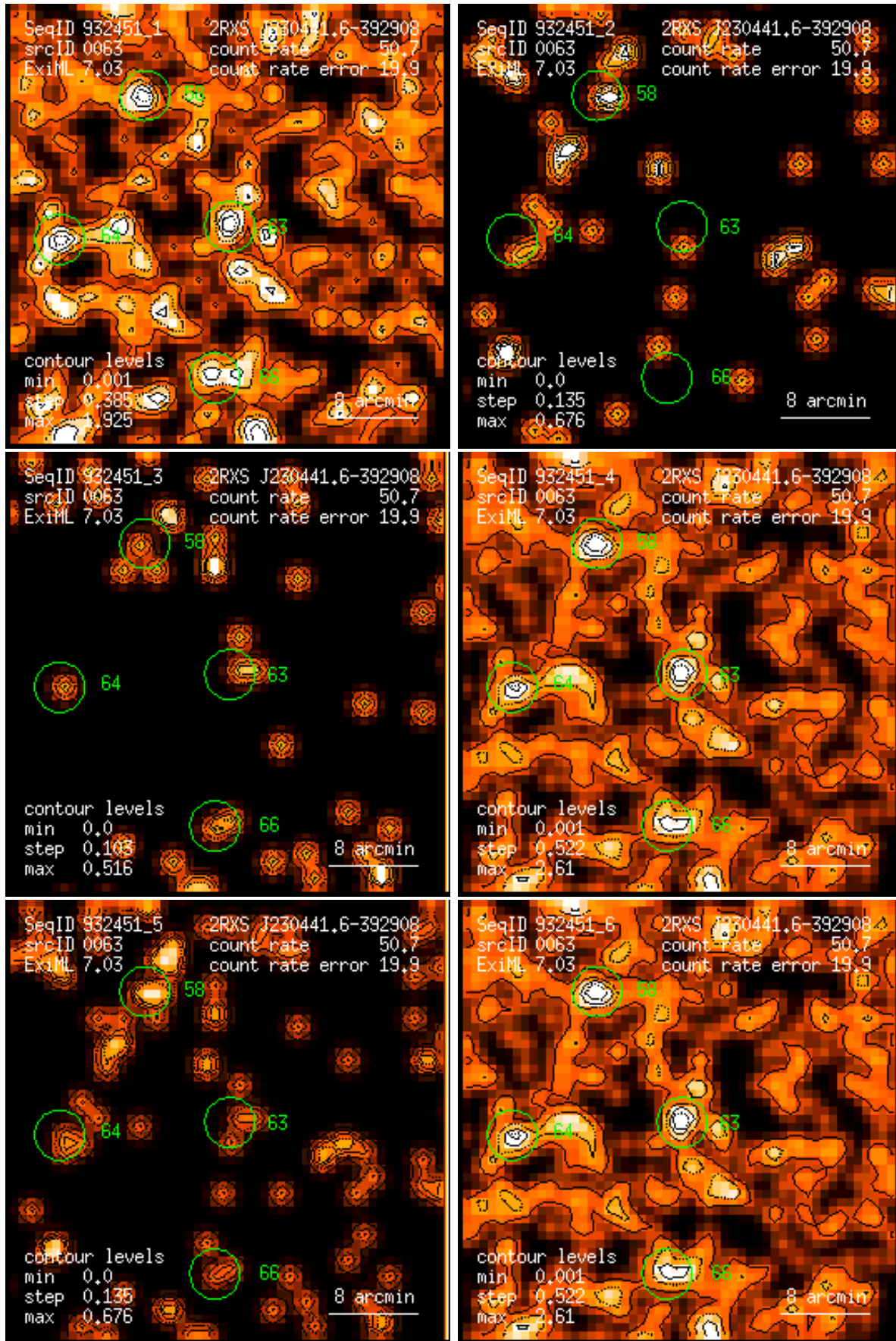
Figure 63: RASS 932451: detection 0063: band rate images, Gaussian filter: (1) PSPC channels 11 – 41, (2) 52 – 90, (3) 91 – 201, (4) 11 – 235, (5) 52 – 201, (6) 11 – 201. Broad band rates in counts/ks. Band rate contour levels in counts/ks/arcmin 2 .
