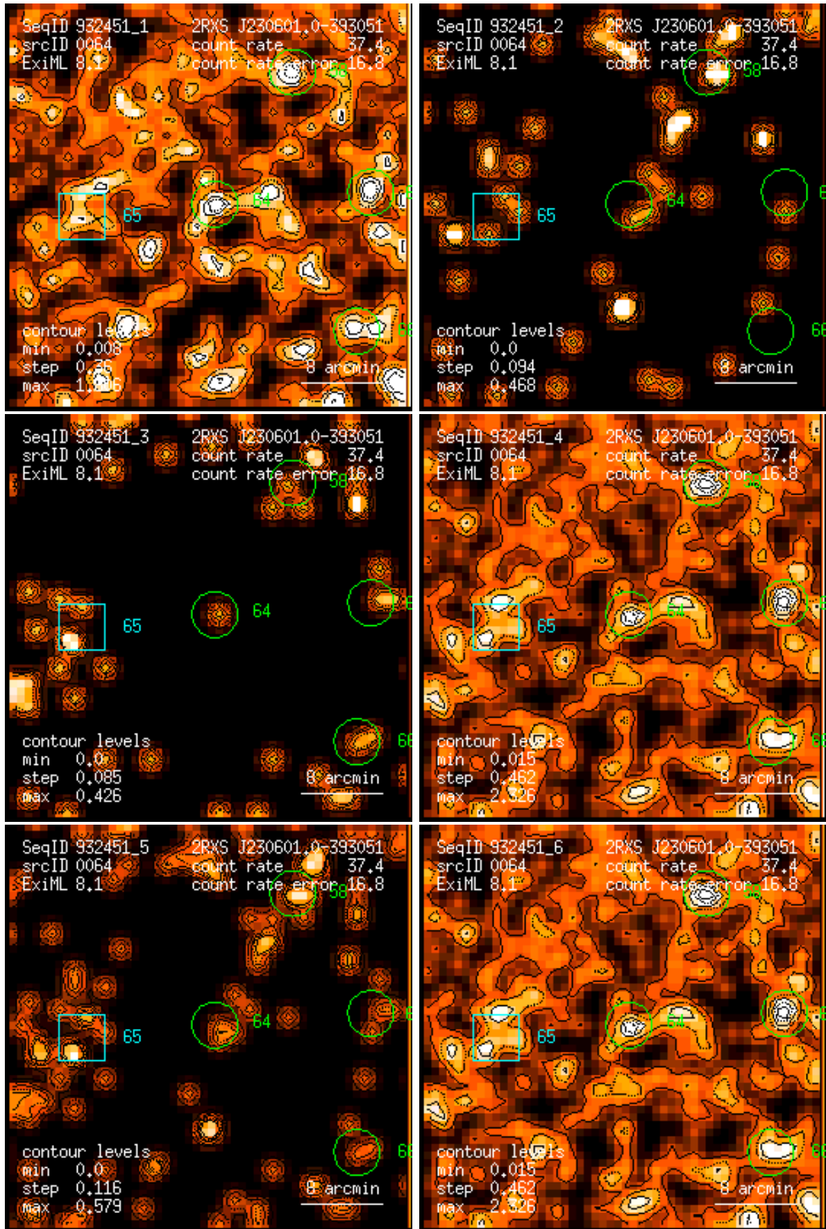
Figure 64: RASS 932451: detection 0064: band rate images, Gaussian filter: (1) PSPC channels 11 – 41, (2) 52 – 90, (3) 91 – 201, (4) 11 – 235, (5) 52 – 201, (6) 11 – 201. Broad band rates in counts/ks. Band rate contour levels in counts/ks/arcmin 2 .
