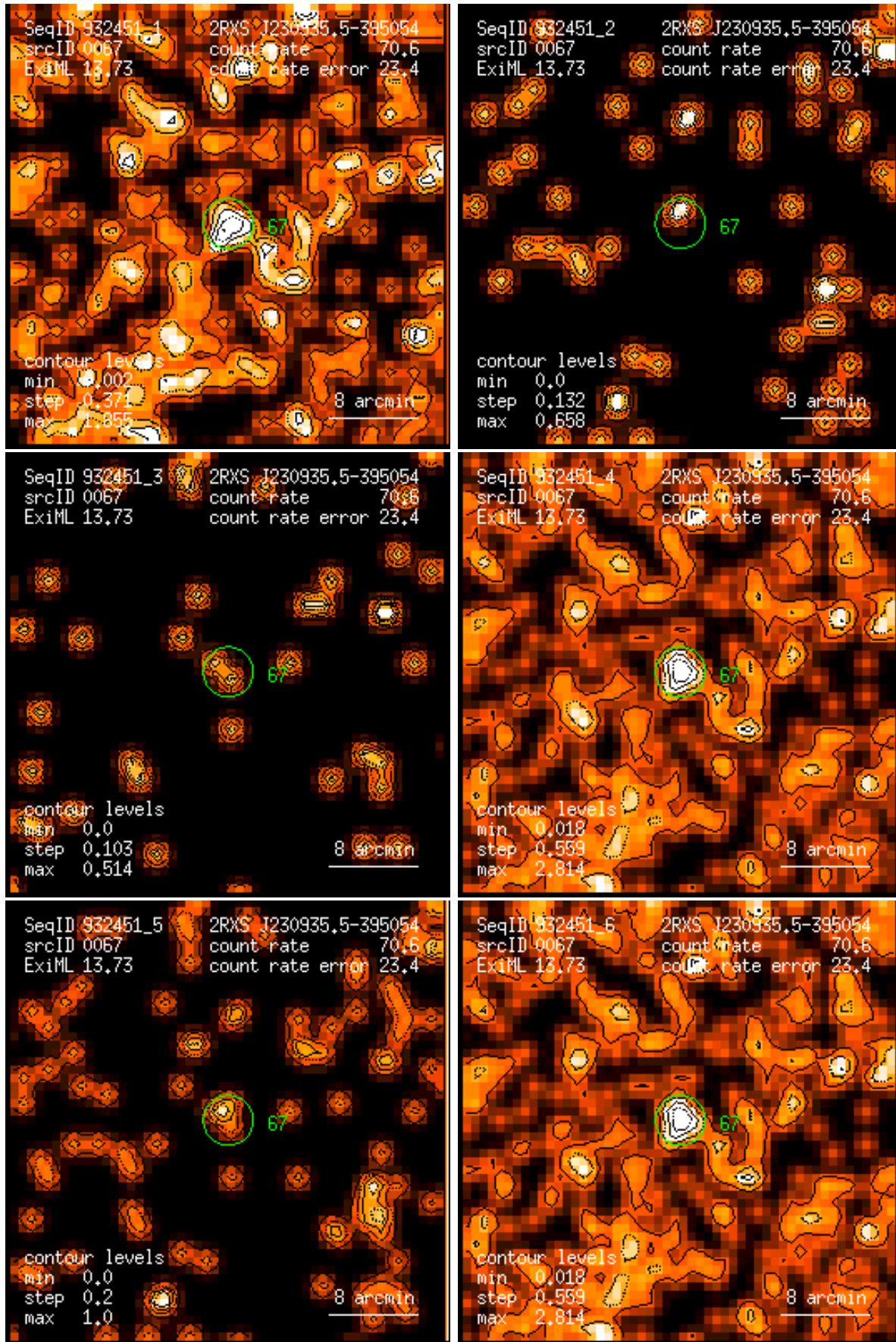
Figure 67: RASS 932451: detection 0067: band rate images, Gaussian filter: (1) PSPC channels 11 – 41, (2) 52 – 90, (3) 91 – 201, (4) 11 – 235, (5) 52 – 201, (6) 11 – 201. Broad band rates in counts/ks. Band rate contour levels in counts/ks/arcmin 2 .
