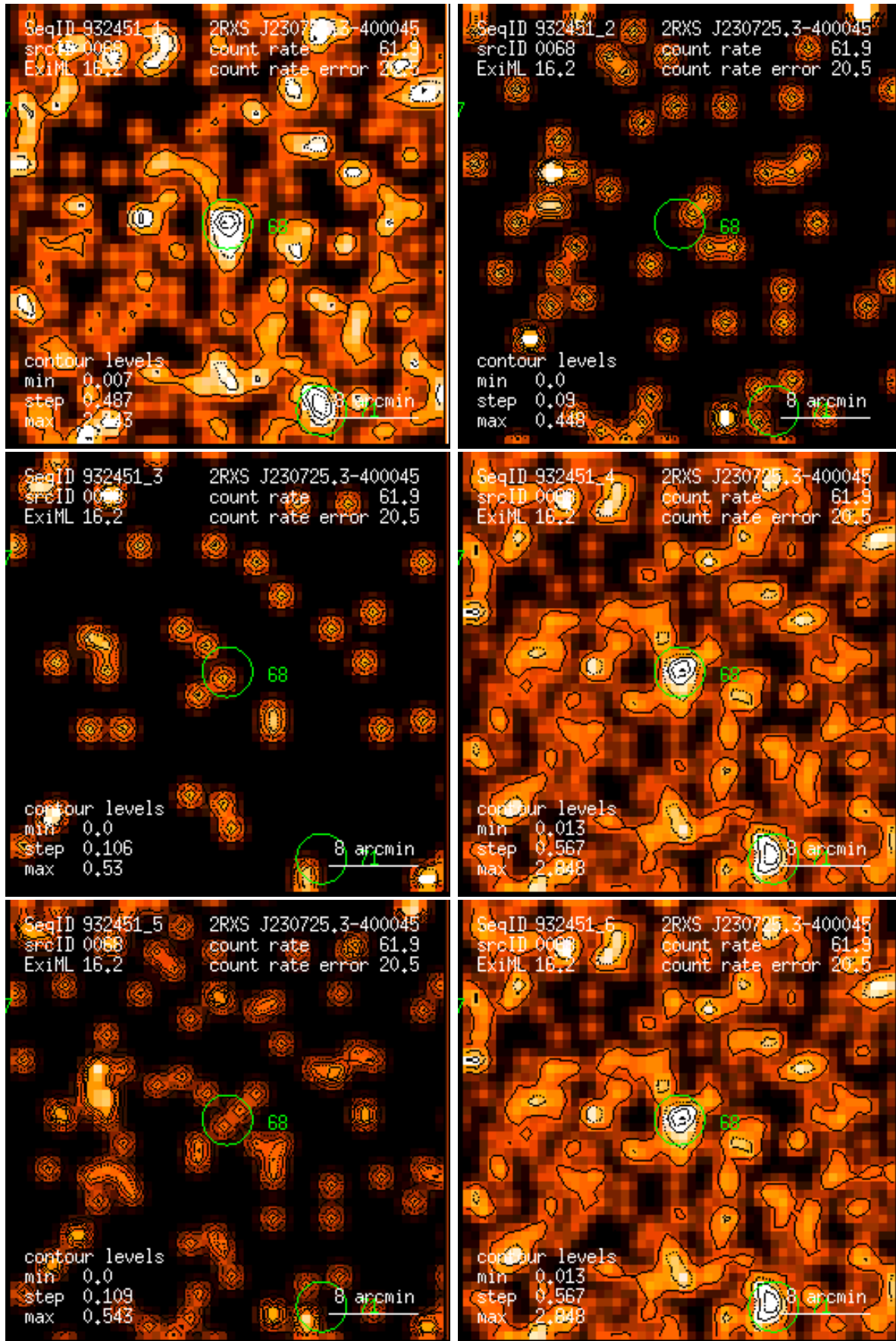
Figure 68: RASS 932451: detection 0068: band rate images, Gaussian filter: (1) PSPC channels 11 – 41, (2) 52 – 90, (3) 91 – 201, (4) 11 – 235, (5) 52 – 201, (6) 11 – 201. Broad band rates in counts/ks. Band rate contour levels in counts/ks/arcmin 2 .
