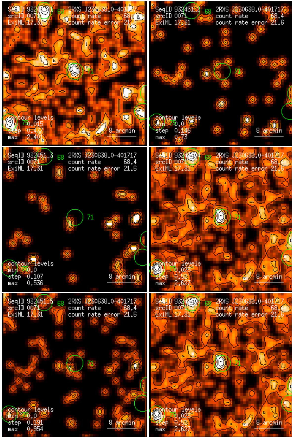
Figure 71: RASS 932451: detection 0071: band rate images, Gaussian filter: (1) PSPC channels 11 – 41, (2) 52 – 90, (3) 91 – 201, (4) 11 – 235, (5) 52 – 201, (6) 11 – 201. Broad band rates in counts/ks. Band rate contour levels in counts/ks/arcmin 2 .
