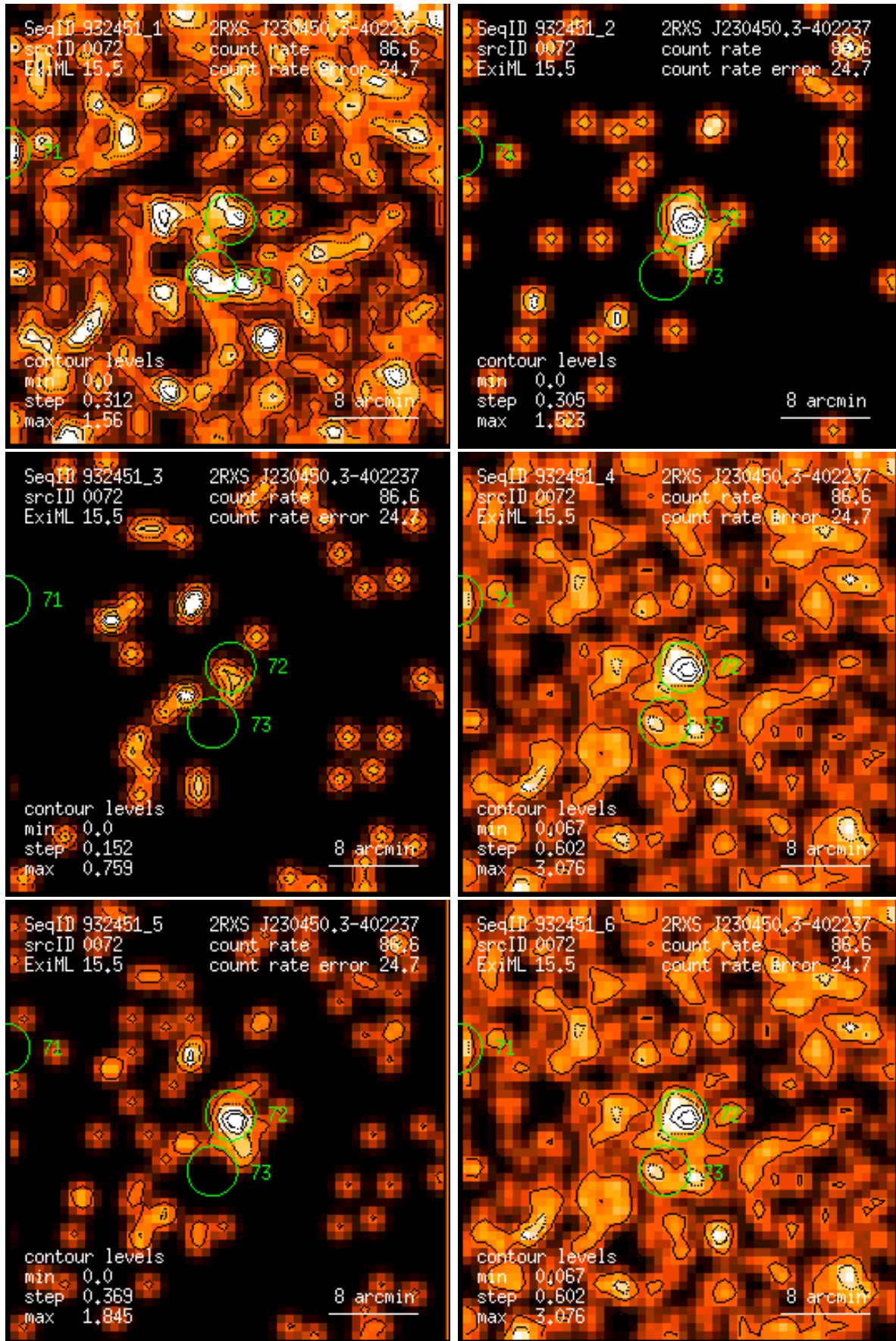
Figure 72: RASS 932451: detection 0072: band rate images, Gaussian filter: (1) PSPC channels 11 – 41, (2) 52 – 90, (3) 91 – 201, (4) 11 – 235, (5) 52 – 201, (6) 11 – 201. Broad band rates in counts/ks. Band rate contour levels in counts/ks/arcmin 2 .
