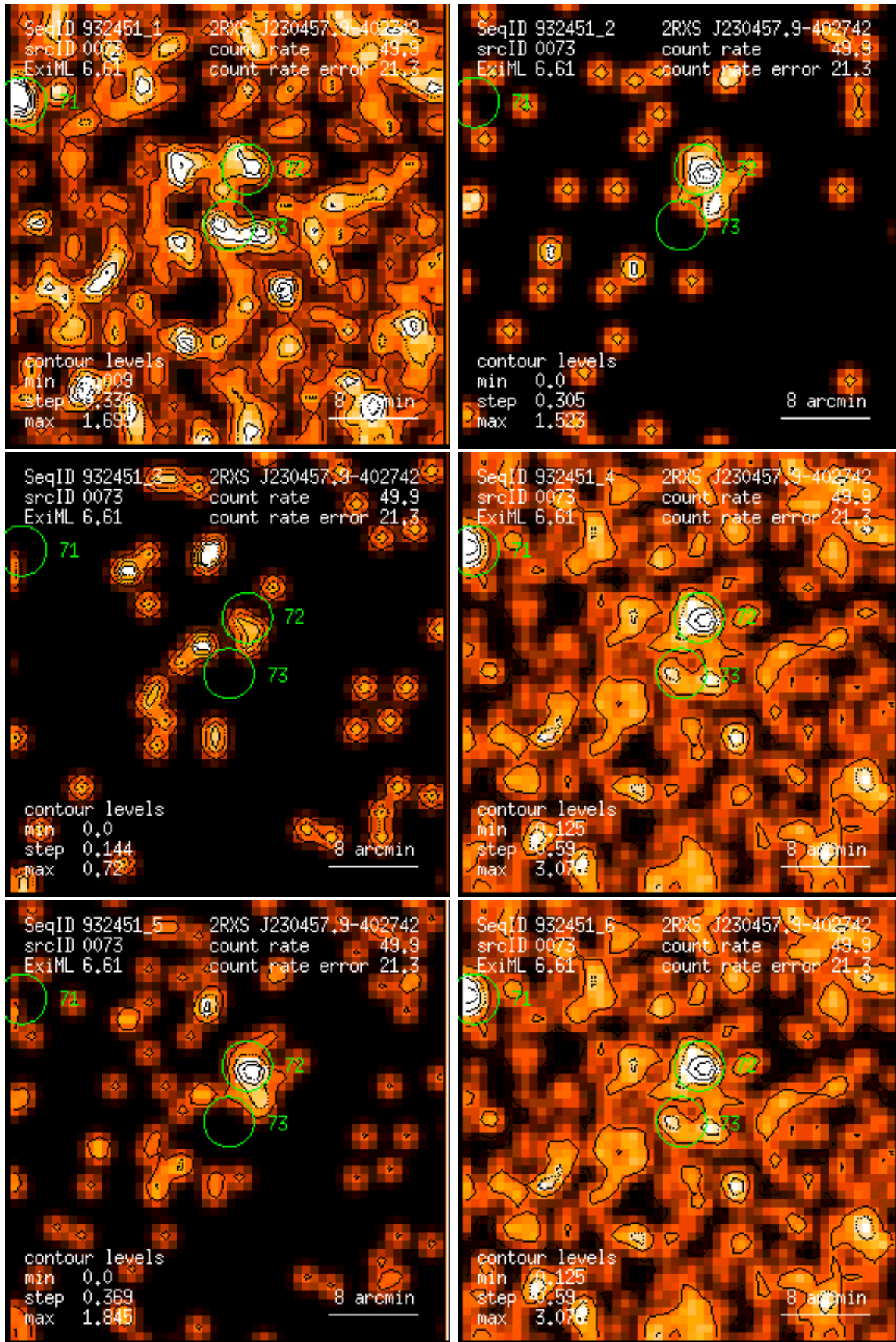
Figure 73: RASS 932451: detection 0073: band rate images, Gaussian filter: (1) PSPC channels 11 – 41, (2) 52 – 90, (3) 91 – 201, (4) 11 – 235, (5) 52 – 201, (6) 11 – 201. Broad band rates in counts/ks. Band rate contour levels in counts/ks/arcmin 2 .
