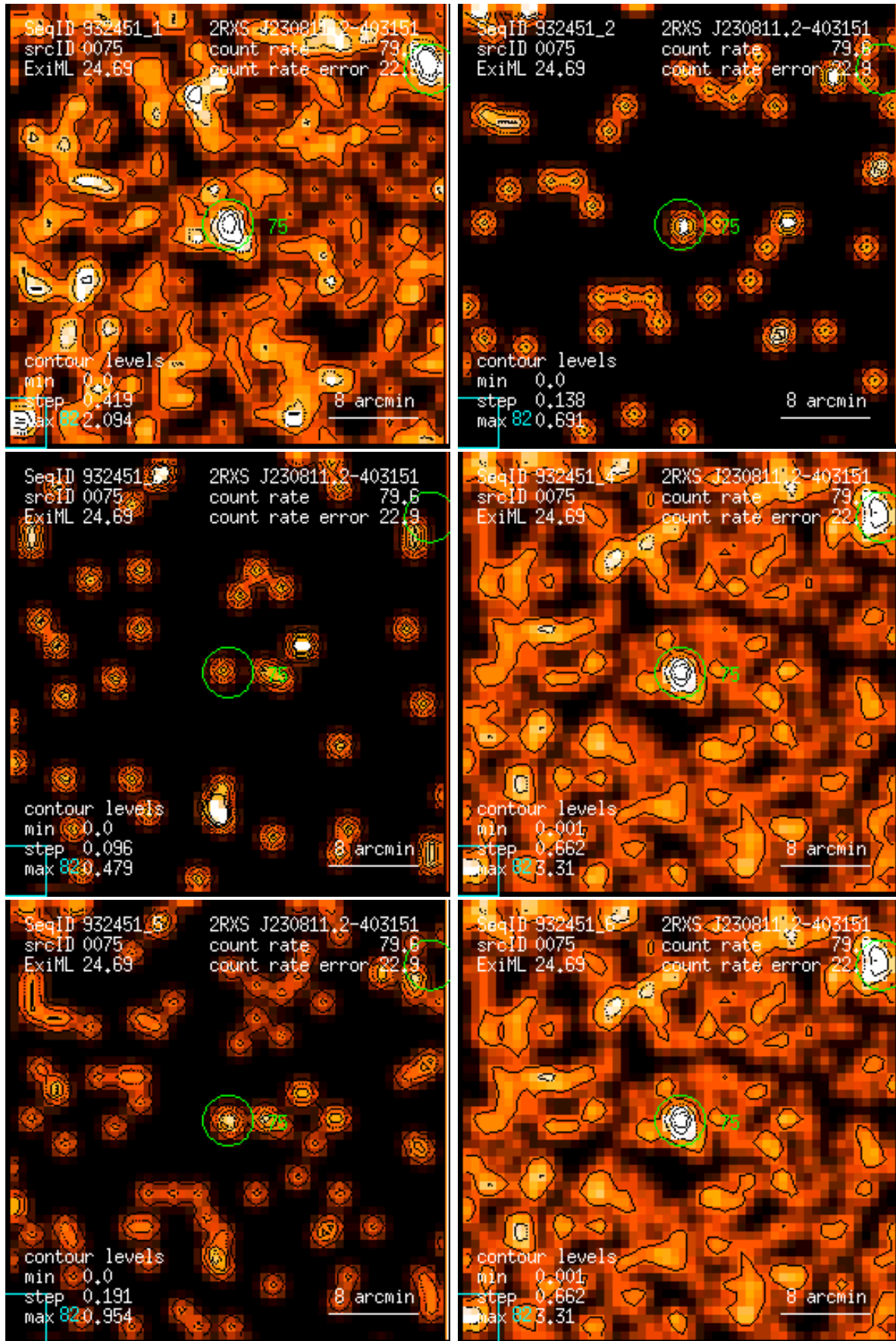
Figure 75: RASS 932451: detection 0075: band rate images, Gaussian filter: (1) PSPC channels 11 – 41, (2) 52 – 90, (3) 91 – 201, (4) 11 – 235, (5) 52 – 201, (6) 11 – 201. Broad band rates in counts/ks. Band rate contour levels in counts/ks/arcmin 2 .
