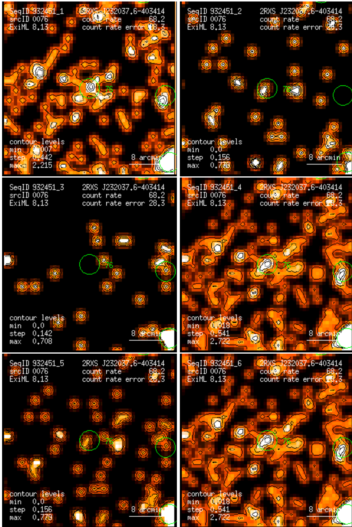
Figure 76: RASS 932451: detection 0076: band rate images, Gaussian filter: (1) PSPC channels 11 – 41, (2) 52 – 90, (3) 91 – 201, (4) 11 – 235, (5) 52 – 201, (6) 11 – 201. Broad band rates in counts/ks. Band rate contour levels in counts/ks/arcmin 2 .
