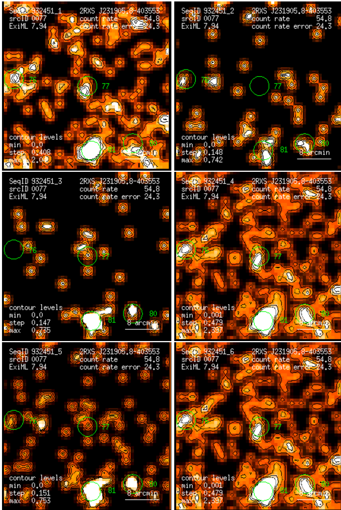
Figure 77: RASS 932451: detection 0077: band rate images, Gaussian filter: (1) PSPC channels 11 – 41, (2) 52 – 90, (3) 91 – 201, (4) 11 – 235, (5) 52 – 201, (6) 11 – 201. Broad band rates in counts/ks. Band rate contour levels in counts/ks/arcmin 2 .
