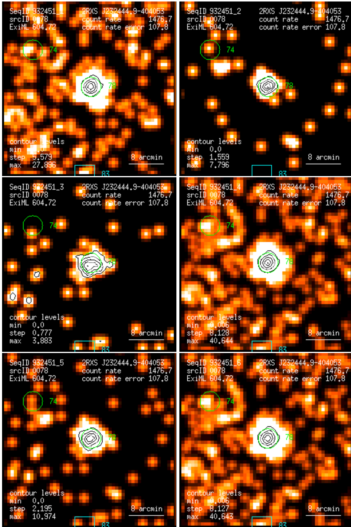
Figure 78: RASS 932451: detection 0078: band rate images, Gaussian filter: (1) PSPC channels 11 – 41, (2) 52 – 90, (3) 91 – 201, (4) 11 – 235, (5) 52 – 201, (6) 11 – 201. Broad band rates in counts/ks. Band rate contour levels in counts/ks/arcmin 2 .
