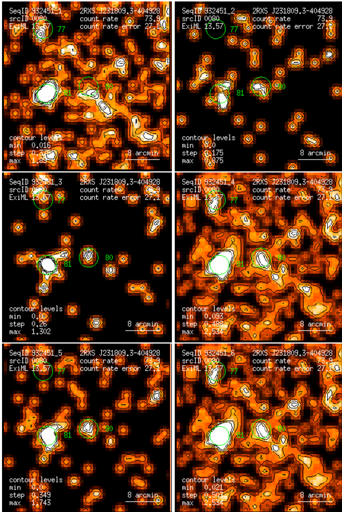
Figure 80: RASS 932451: detection 0080: band rate images, Gaussian filter: (1) PSPC channels 11 – 41, (2) 52 – 90, (3) 91 – 201, (4) 11 – 235, (5) 52 – 201, (6) 11 – 201. Broad band rates in counts/ks. Band rate contour levels in counts/ks/arcmin 2 .
