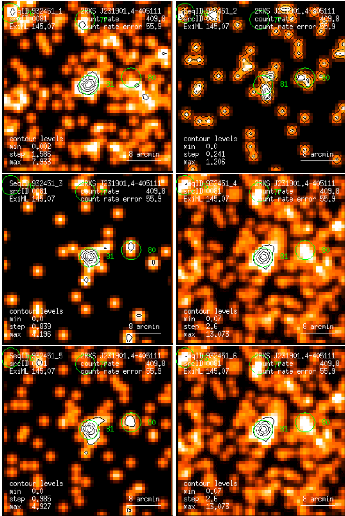
Figure 81: RASS 932451: detection 0081: band rate images, Gaussian filter: (1) PSPC channels 11 – 41, (2) 52 – 90, (3) 91 – 201, (4) 11 – 235, (5) 52 – 201, (6) 11 – 201. Broad band rates in counts/ks. Band rate contour levels in counts/ks/arcmin 2 .
