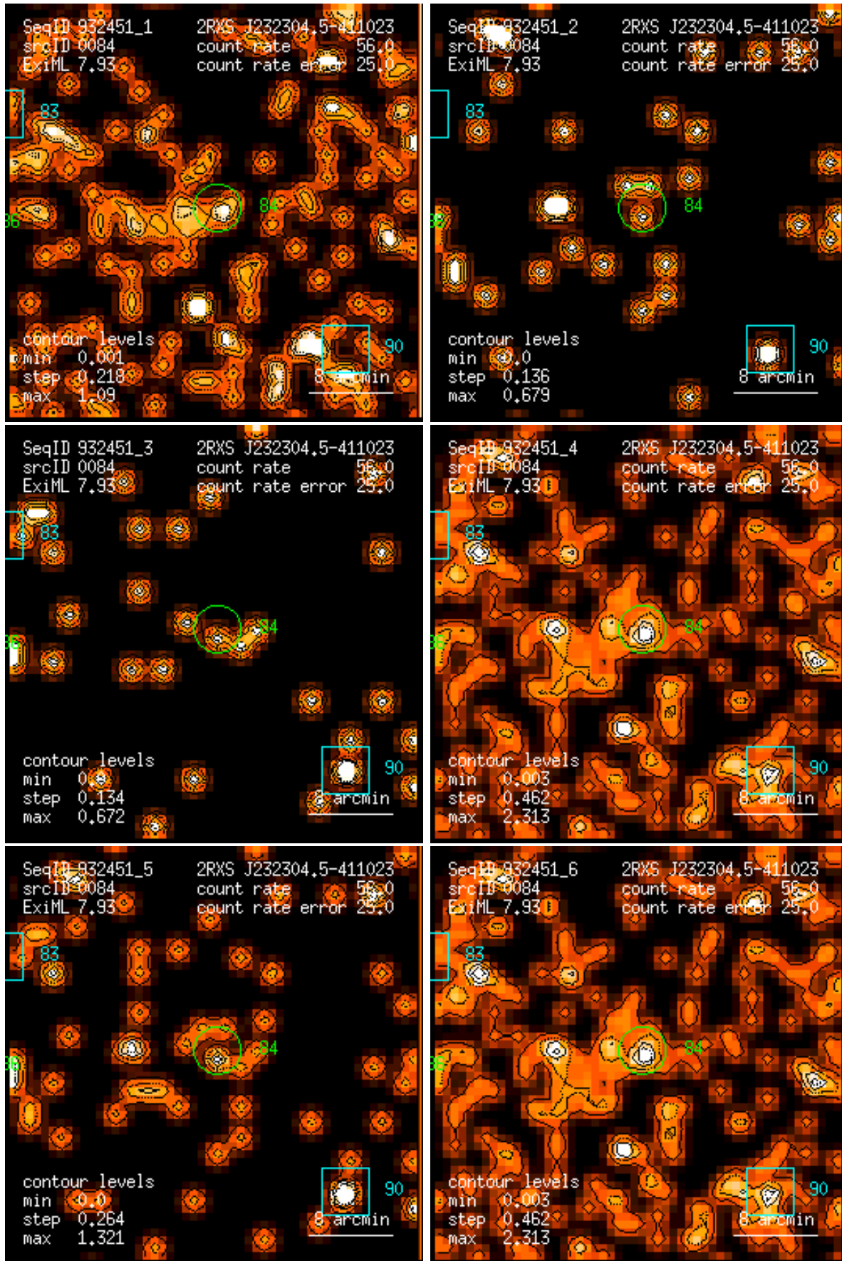
Figure 84: RASS 932451: detection 0084: band rate images, Gaussian filter: (1) PSPC channels 11 – 41, (2) 52 – 90, (3) 91 – 201, (4) 11 – 235, (5) 52 – 201, (6) 11 – 201. Broad band rates in counts/ks. Band rate contour levels in counts/ks/arcmin 2 .
