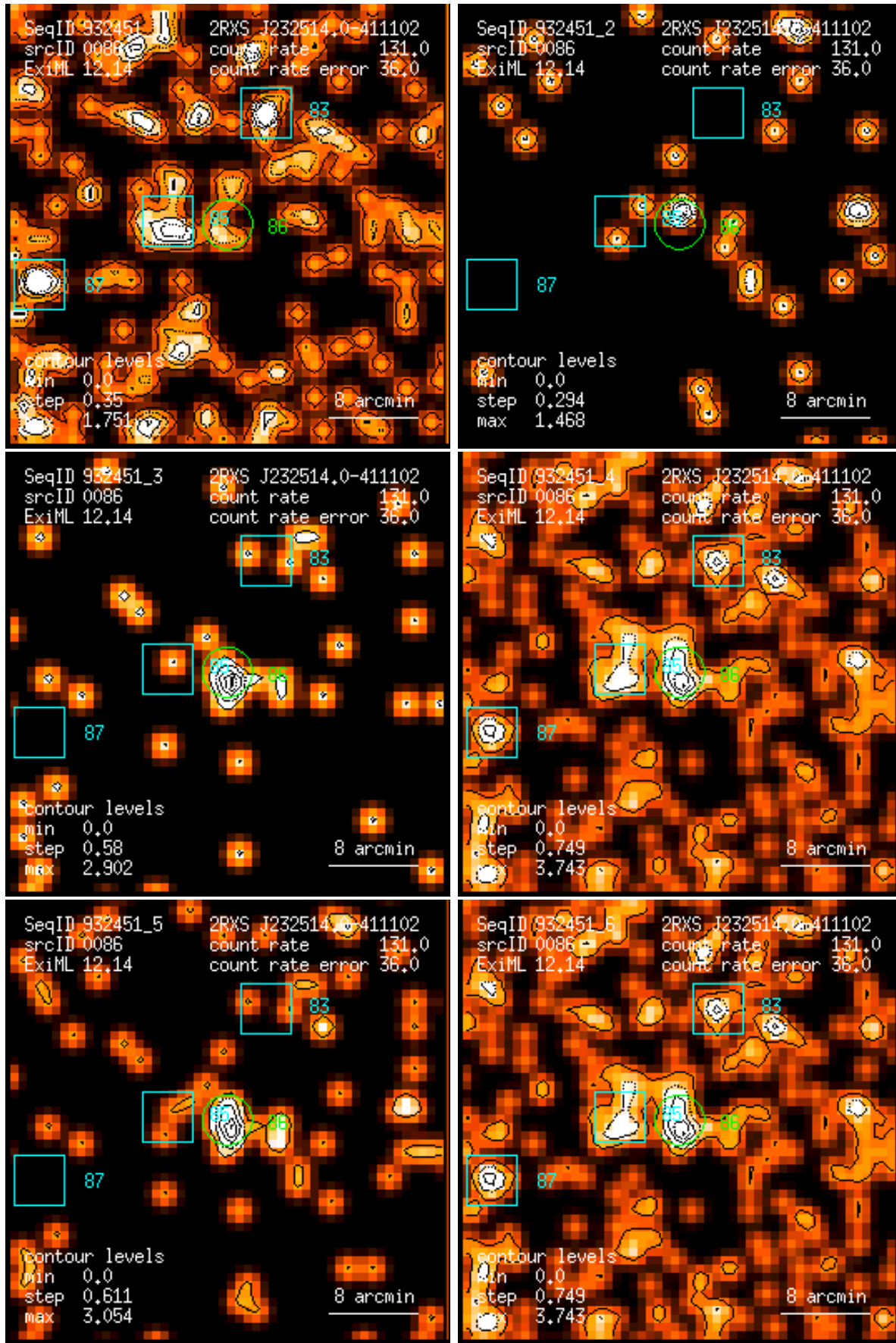
Figure 86: RASS 932451: detection 0086: band rate images, Gaussian filter: (1) PSPC channels 11 – 41, (2) 52 – 90, (3) 91 – 201, (4) 11 – 235, (5) 52 – 201, (6) 11 – 201. Broad band rates in counts/ks. Band rate contour levels in counts/ks/arcmin 2 .
