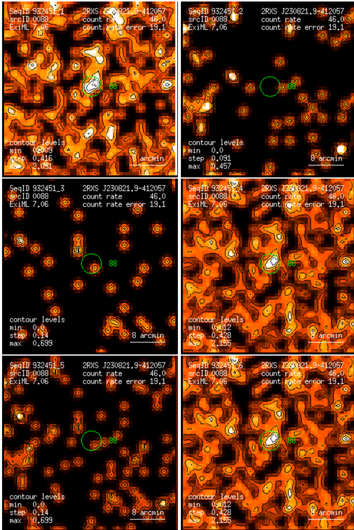
Figure 88: RASS 932451: detection 0088: band rate images, Gaussian filter: (1) PSPC channels 11 – 41, (2) 52 – 90, (3) 91 – 201, (4) 11 – 235, (5) 52 – 201, (6) 11 – 201. Broad band rates in counts/ks. Band rate contour levels in counts/ks/arcmin 2 .
