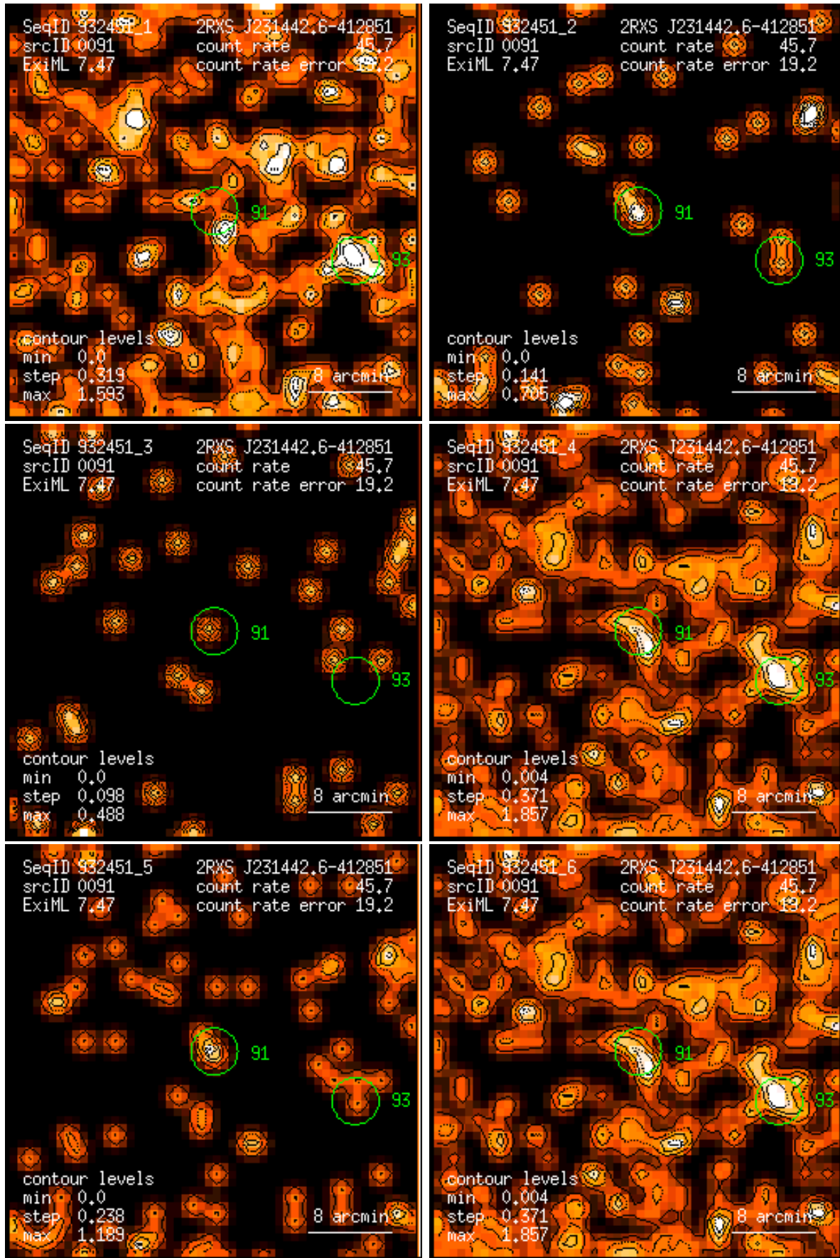
Figure 91: RASS 932451: detection 0091: band rate images, Gaussian filter: (1) PSPC channels 11 – 41, (2) 52 – 90, (3) 91 – 201, (4) 11 – 235, (5) 52 – 201, (6) 11 – 201. Broad band rates in counts/ks. Band rate contour levels in counts/ks/arcmin 2 .
