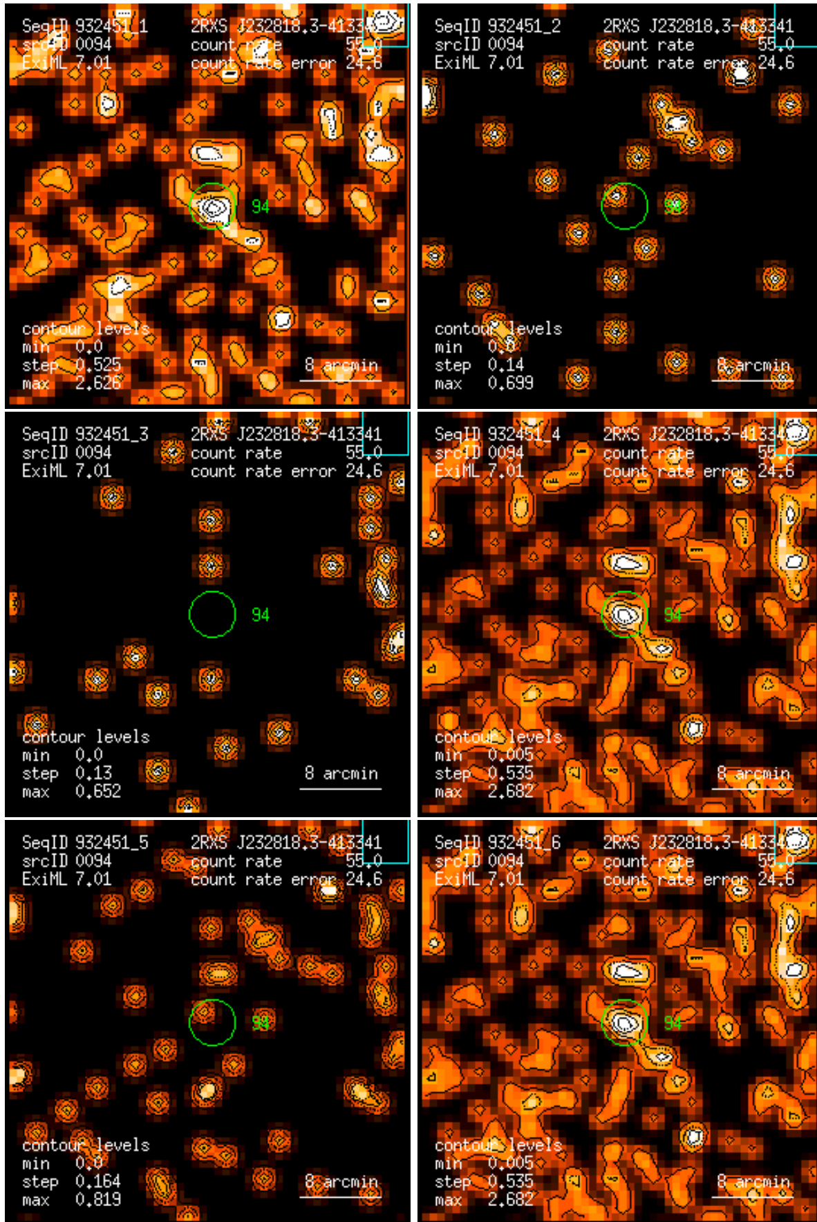
Figure 94: RASS 932451: detection 0094: band rate images, Gaussian filter: (1) PSPC channels 11 – 41, (2) 52 – 90, (3) 91 – 201, (4) 11 – 235, (5) 52 – 201, (6) 11 – 201. Broad band rates in counts/ks. Band rate contour levels in counts/ks/arcmin 2 .
